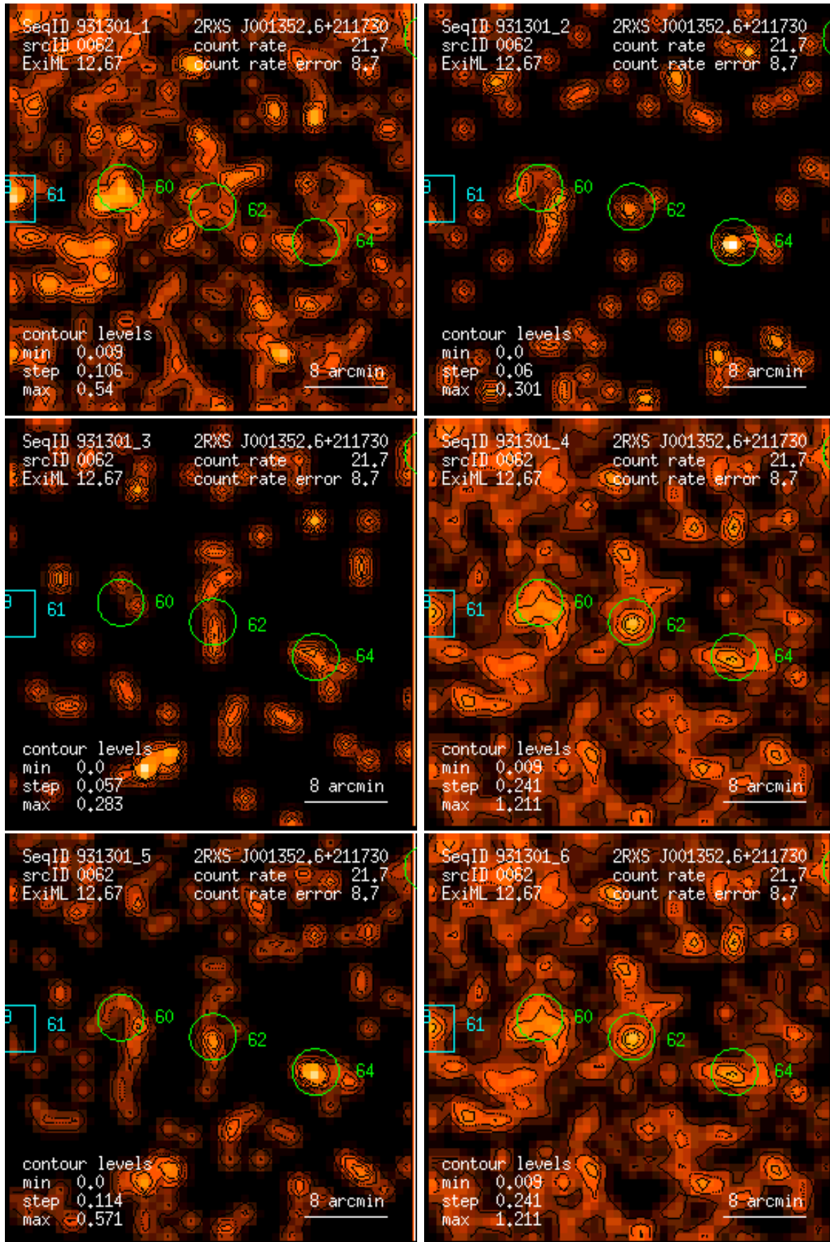
Figure 62: RASS 931301: detection 0062: band rate images, Gaussian filter: (1) PSPC channels 11 – 41, (2) 52 – 90, (3) 91 – 201, (4) 11 – 235, (5) 52 – 201, (6) 11 – 201. Broad band rates in counts/ks. Band rate contour levels in counts/ks/arcmin 2 .
