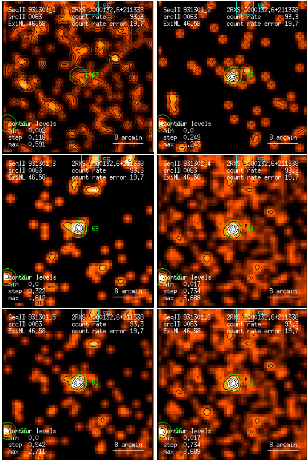
Figure 63: RASS 931301: detection 0063: band rate images, Gaussian filter: (1) PSPC channels 11 – 41, (2) 52 – 90, (3) 91 – 201, (4) 11 – 235, (5) 52 – 201, (6) 11 – 201. Broad band rates in counts/ks. Band rate contour levels in counts/ks/arcmin 2 .
