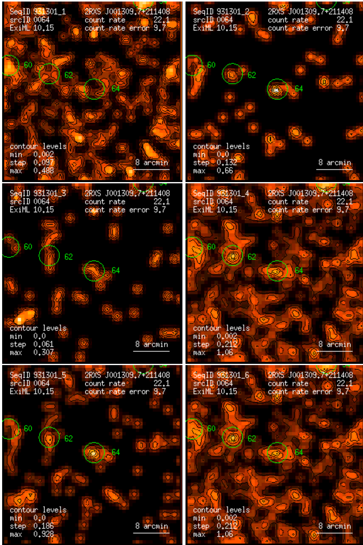
Figure 64: RASS 931301: detection 0064: band rate images, Gaussian filter: (1) PSPC channels 11 – 41, (2) 52 – 90, (3) 91 – 201, (4) 11 – 235, (5) 52 – 201, (6) 11 – 201. Broad band rates in counts/ks. Band rate contour levels in counts/ks/arcmin 2 .
