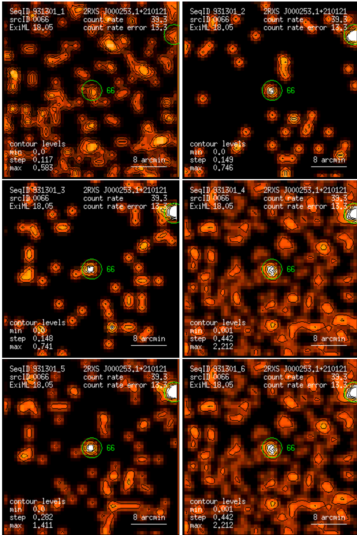
Figure 66: RASS 931301: detection 0066: band rate images, Gaussian filter: (1) PSPC channels 11 – 41, (2) 52 – 90, (3) 91 – 201, (4) 11 – 235, (5) 52 – 201, (6) 11 – 201. Broad band rates in counts/ks. Band rate contour levels in counts/ks/arcmin 2 .
