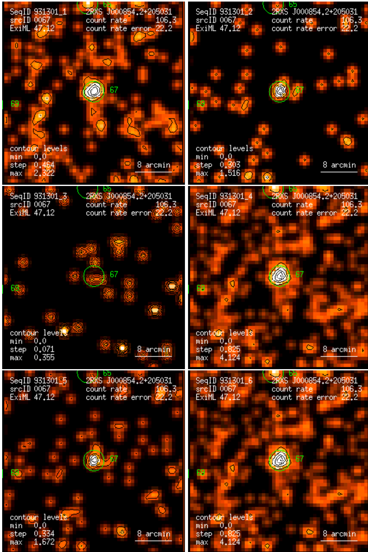
Figure 67: RASS 931301: detection 0067: band rate images, Gaussian filter: (1) PSPC channels 11 – 41, (2) 52 – 90, (3) 91 – 201, (4) 11 – 235, (5) 52 – 201, (6) 11 – 201. Broad band rates in counts/ks. Band rate contour levels in counts/ks/arcmin 2 .
