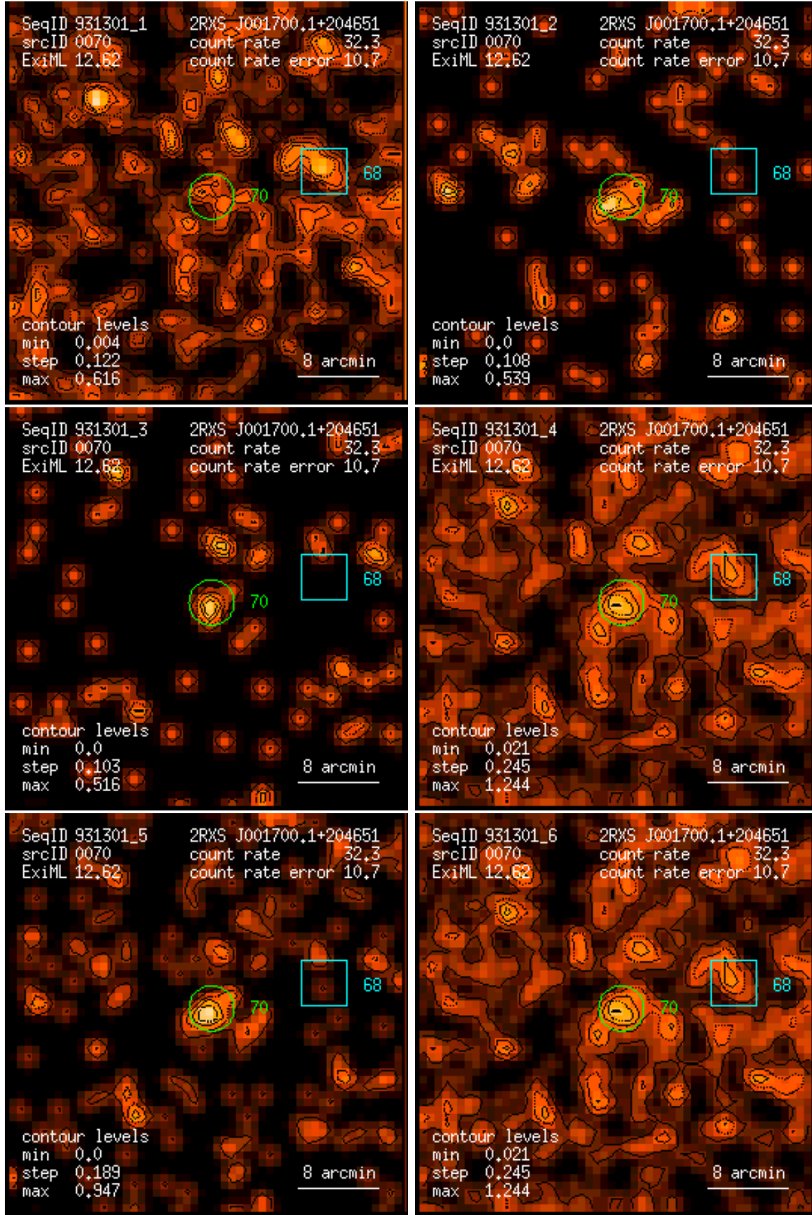
Figure 70: RASS 931301: detection 0070: band rate images, Gaussian filter: (1) PSPC channels 11 – 41, (2) 52 – 90, (3) 91 – 201, (4) 11 – 235, (5) 52 – 201, (6) 11 – 201. Broad band rates in counts/ks. Band rate contour levels in counts/ks/arcmin 2 .
