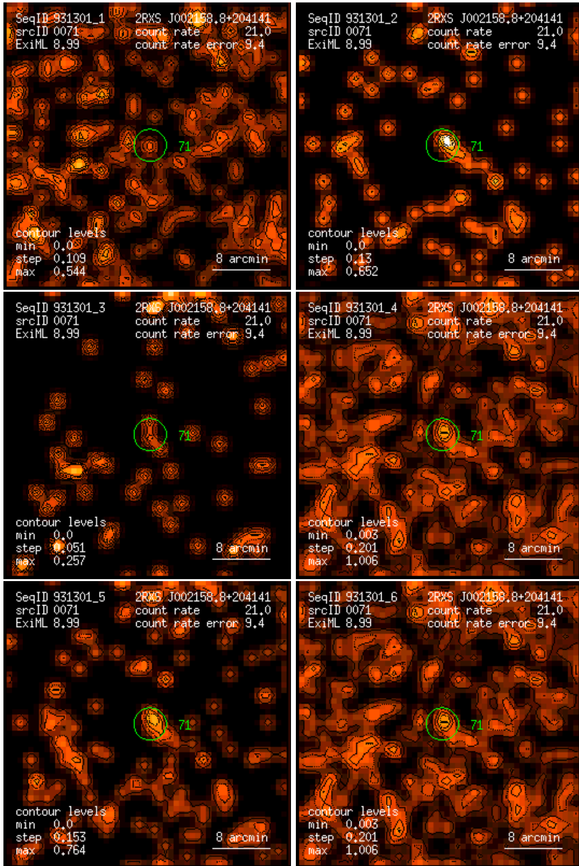
Figure 71: RASS 931301: detection 0071: band rate images, Gaussian filter: (1) PSPC channels 11 – 41, (2) 52 – 90, (3) 91 – 201, (4) 11 – 235, (5) 52 – 201, (6) 11 – 201. Broad band rates in counts/ks. Band rate contour levels in counts/ks/arcmin 2 .
