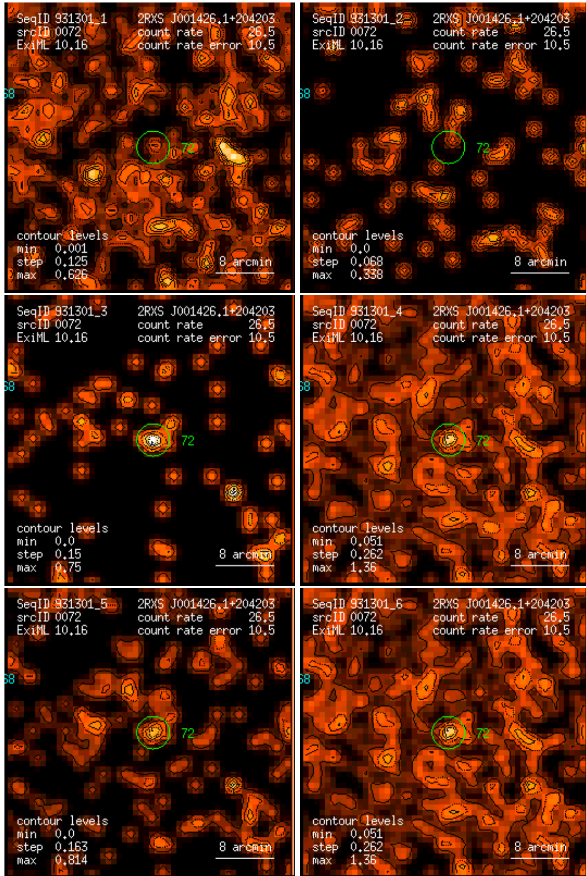
Figure 72: RASS 931301: detection 0072: band rate images, Gaussian filter: (1) PSPC channels 11 – 41, (2) 52 – 90, (3) 91 – 201, (4) 11 – 235, (5) 52 – 201, (6) 11 – 201. Broad band rates in counts/ks. Band rate contour levels in counts/ks/arcmin 2 .
