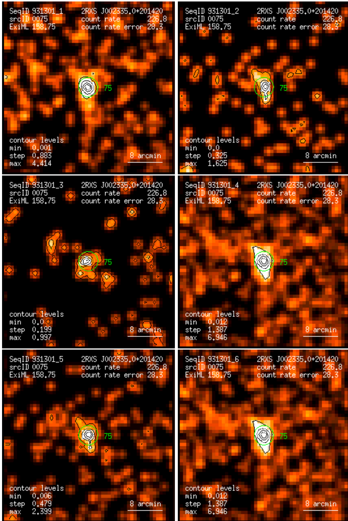
Figure 75: RASS 931301: detection 0075: band rate images, Gaussian filter: (1) PSPC channels 11 – 41, (2) 52 – 90, (3) 91 – 201, (4) 11 – 235, (5) 52 – 201, (6) 11 – 201. Broad band rates in counts/ks. Band rate contour levels in counts/ks/arcmin 2 .
