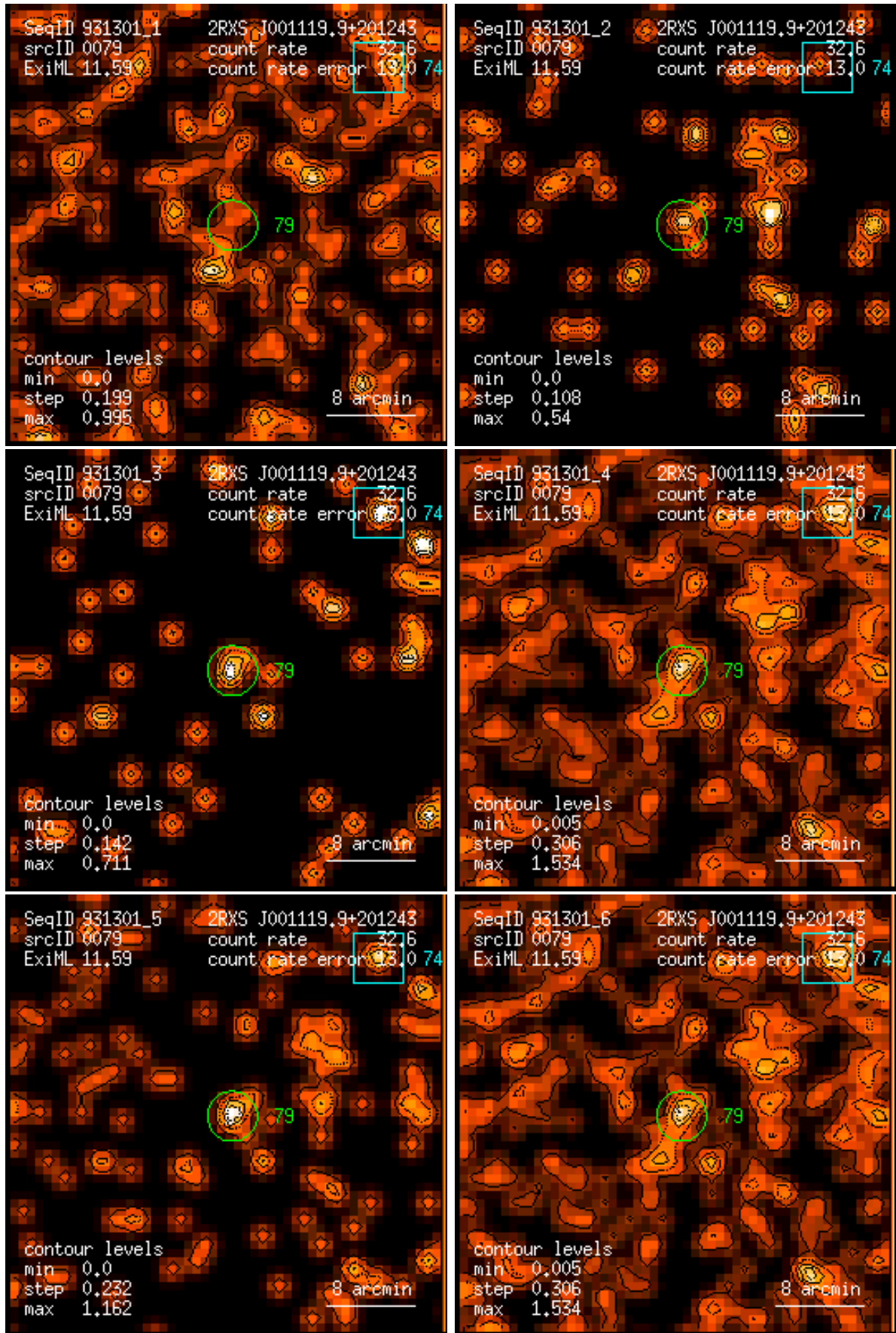
Figure 79: RASS 931301: detection 0079: band rate images, Gaussian filter: (1) PSPC channels 11 – 41, (2) 52 – 90, (3) 91 – 201, (4) 11 – 235, (5) 52 – 201, (6) 11 – 201. Broad band rates in counts/ks. Band rate contour levels in counts/ks/arcmin 2 .
