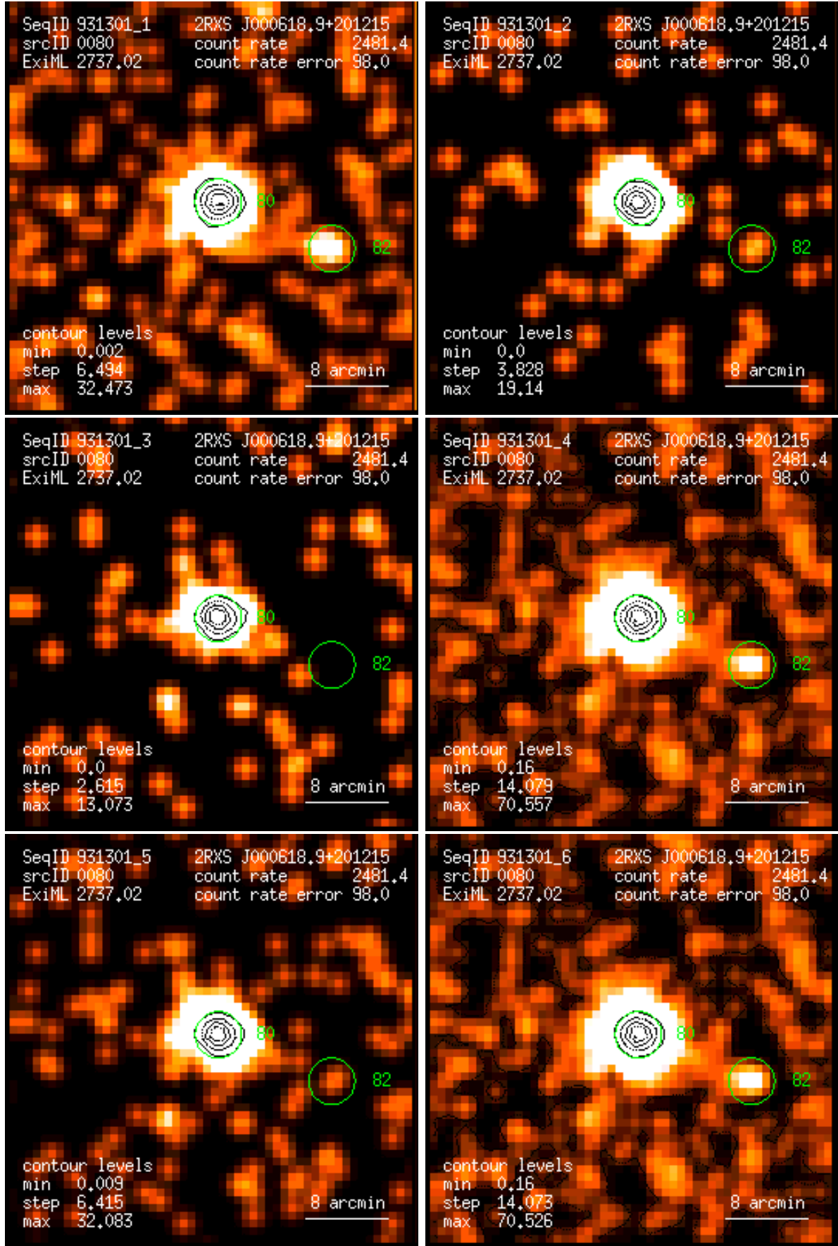
Figure 80: RASS 931301: detection 0080: band rate images, Gaussian filter: (1) PSPC channels 11 – 41, (2) 52 – 90, (3) 91 – 201, (4) 11 – 235, (5) 52 – 201, (6) 11 – 201. Broad band rates in counts/ks. Band rate contour levels in counts/ks/arcmin 2 .
