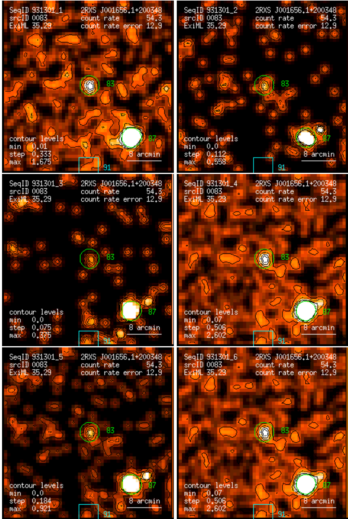
Figure 83: RASS 931301: detection 0083: band rate images, Gaussian filter: (1) PSPC channels 11 – 41, (2) 52 – 90, (3) 91 – 201, (4) 11 – 235, (5) 52 – 201, (6) 11 – 201. Broad band rates in counts/ks. Band rate contour levels in counts/ks/arcmin 2 .
