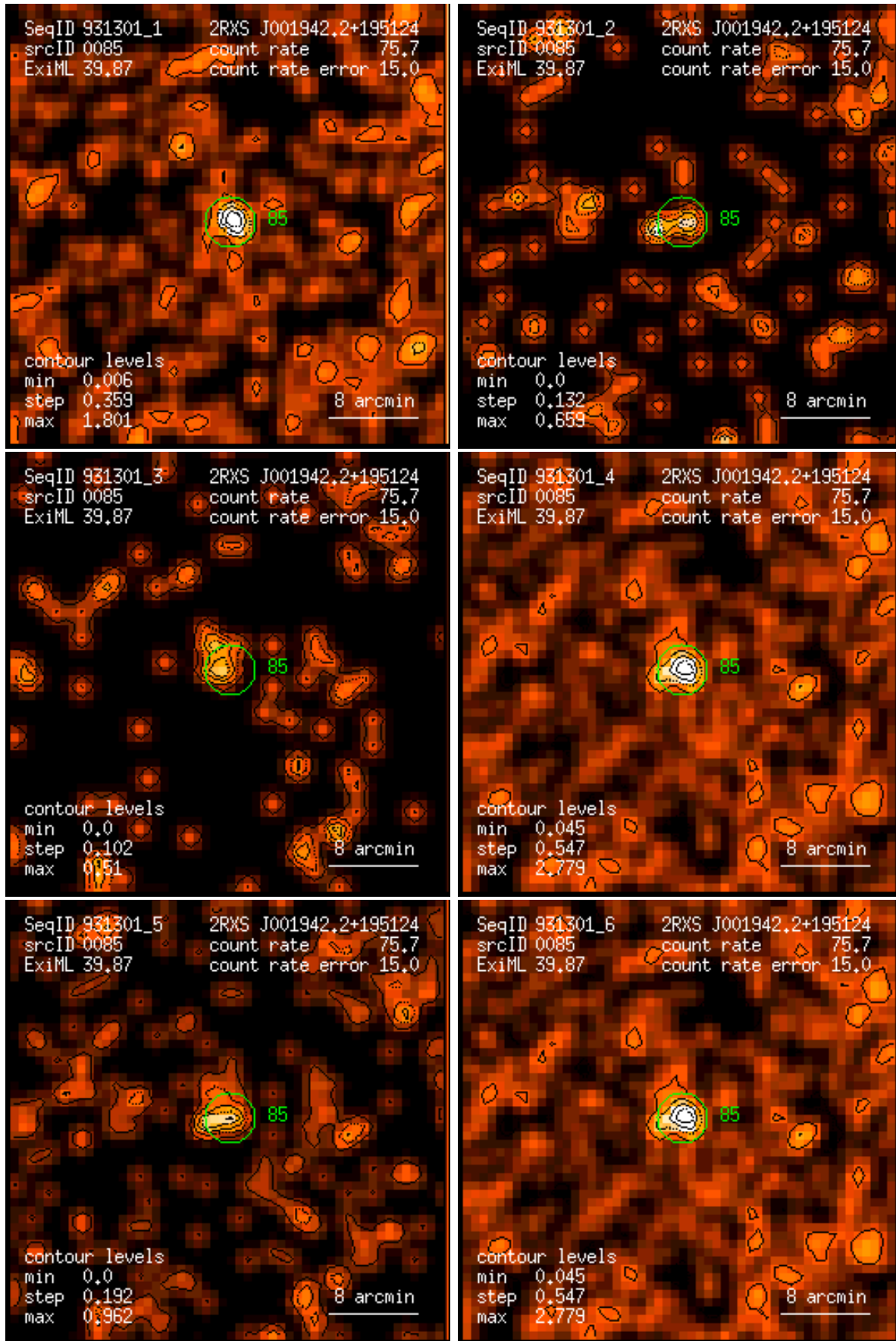
Figure 85: RASS 931301: detection 0085: band rate images, Gaussian filter: (1) PSPC channels 11 – 41, (2) 52 – 90, (3) 91 – 201, (4) 11 – 235, (5) 52 – 201, (6) 11 – 201. Broad band rates in counts/ks. Band rate contour levels in counts/ks/arcmin 2 .
