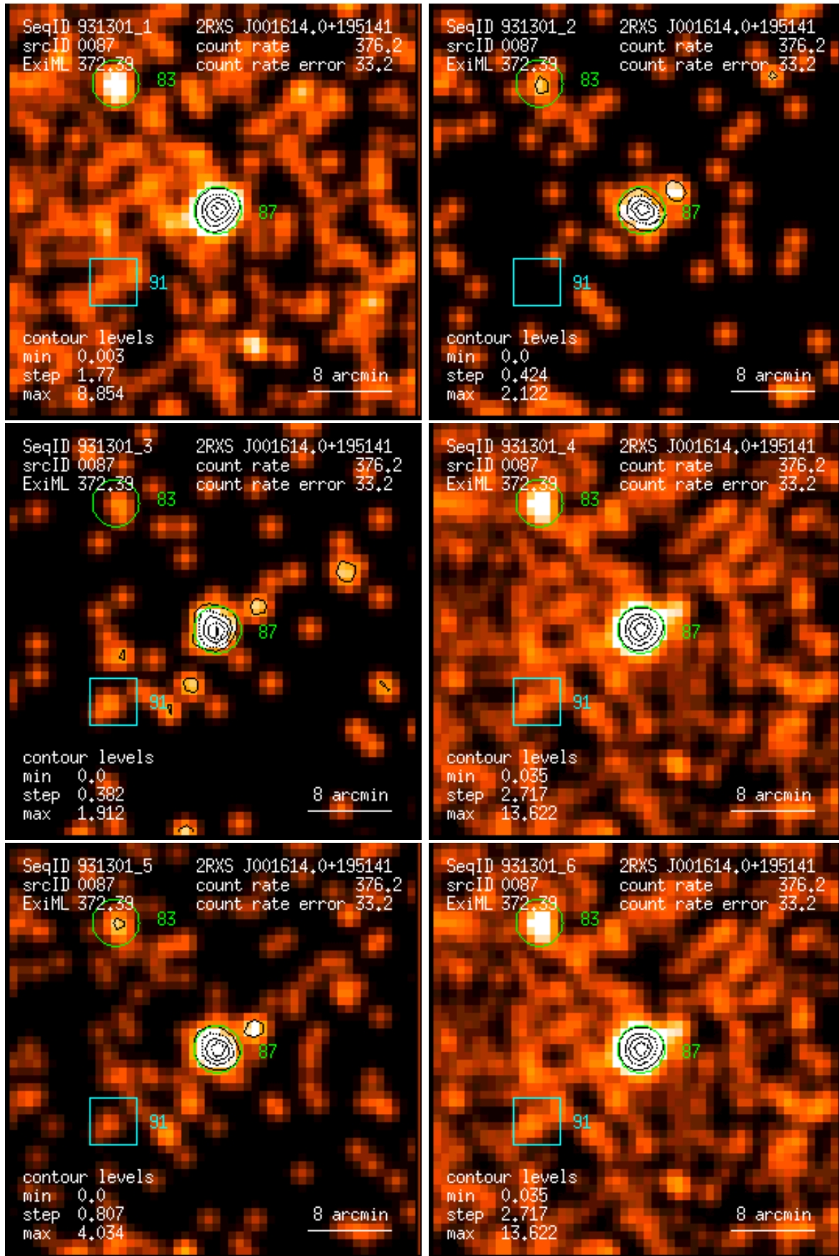
Figure 87: RASS 931301: detection 0087: band rate images, Gaussian filter: (1) PSPC channels 11 – 41, (2) 52 – 90, (3) 91 – 201, (4) 11 – 235, (5) 52 – 201, (6) 11 – 201. Broad band rates in counts/ks. Band rate contour levels in counts/ks/arcmin 2 .
