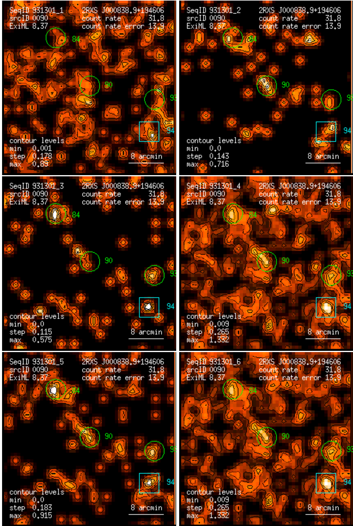
Figure 90: RASS 931301: detection 0090: band rate images, Gaussian filter: (1) PSPC channels 11 – 41, (2) 52 – 90, (3) 91 – 201, (4) 11 – 235, (5) 52 – 201, (6) 11 – 201. Broad band rates in counts/ks. Band rate contour levels in counts/ks/arcmin 2 .
