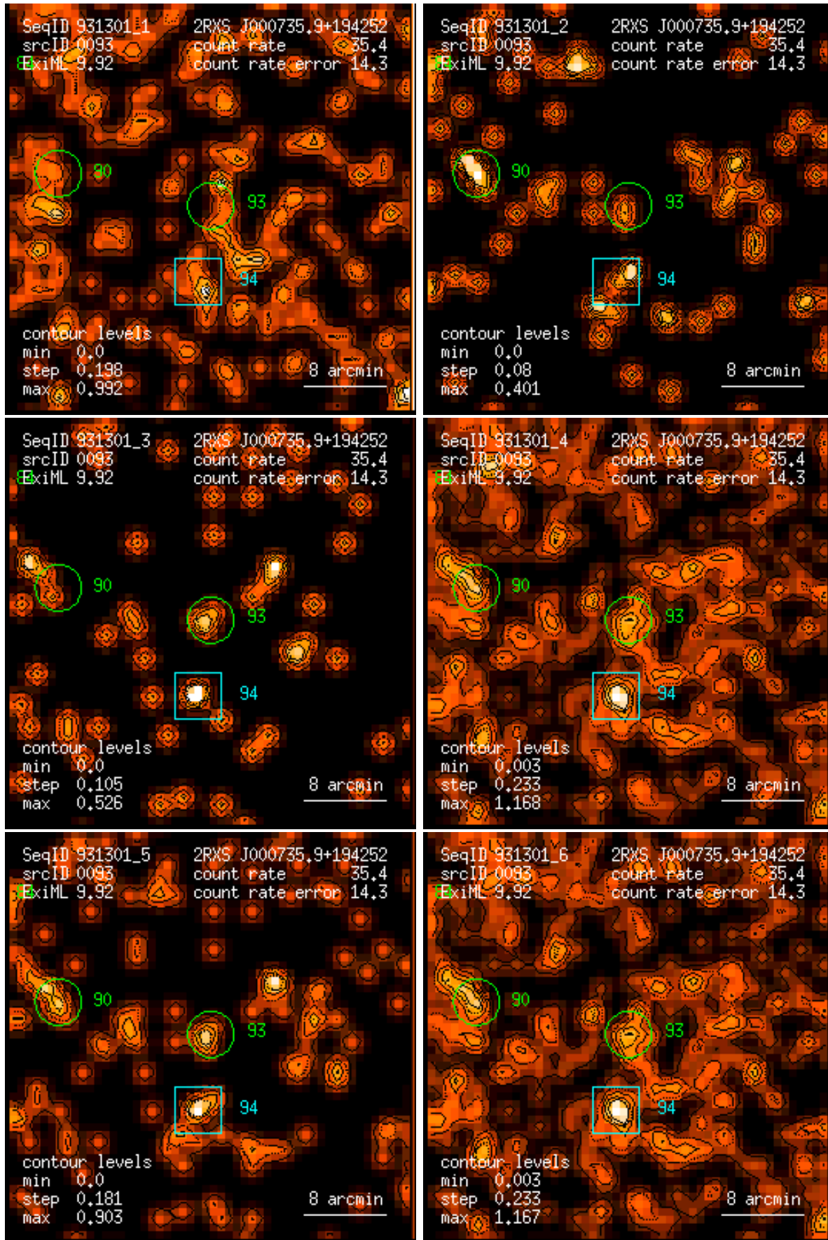
Figure 93: RASS 931301: detection 0093: band rate images, Gaussian filter: (1) PSPC channels 11 – 41, (2) 52 – 90, (3) 91 – 201, (4) 11 – 235, (5) 52 – 201, (6) 11 – 201. Broad band rates in counts/ks. Band rate contour levels in counts/ks/arcmin 2 .
