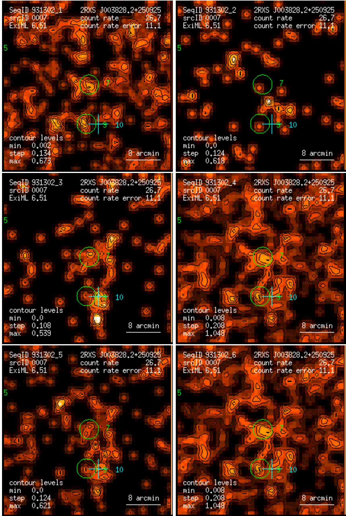
Figure 7: RASS 931302: detection 0007: band rate images, Gaussian filter: (1) PSPC channels 11 – 41, (2) 52 – 90, (3) 91 – 201, (4) 11 – 235, (5) 52 – 201, (6) 11 – 201. Broad band rates in counts/ks. Band rate contour levels in counts/ks/arcmin 2 .
