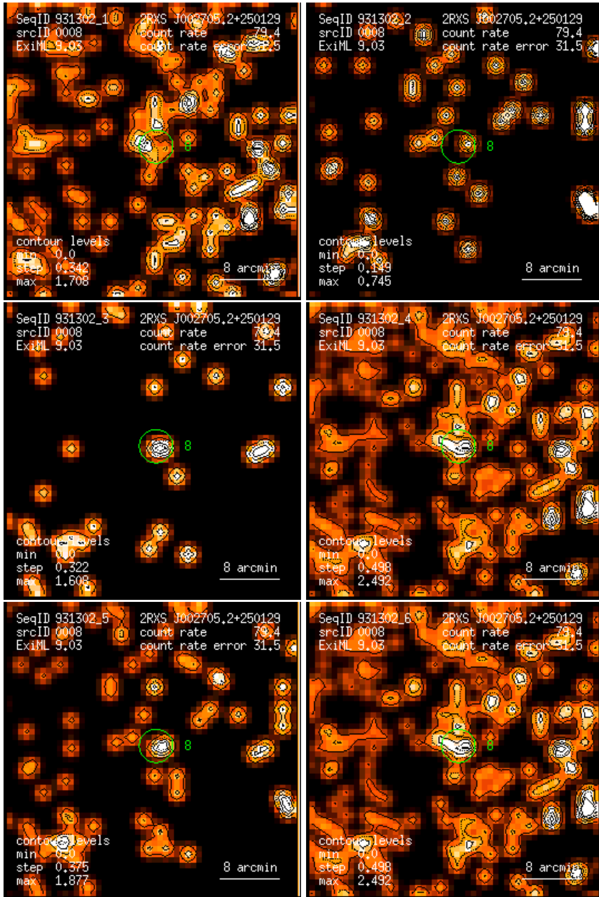
Figure 8: RASS 931302: detection 0008: band rate images, Gaussian filter: (1) PSPC channels 11 – 41, (2) 52 – 90, (3) 91 – 201, (4) 11 – 235, (5) 52 – 201, (6) 11 – 201. Broad band rates in counts/ks. Band rate contour levels in counts/ks/arcmin 2 .
