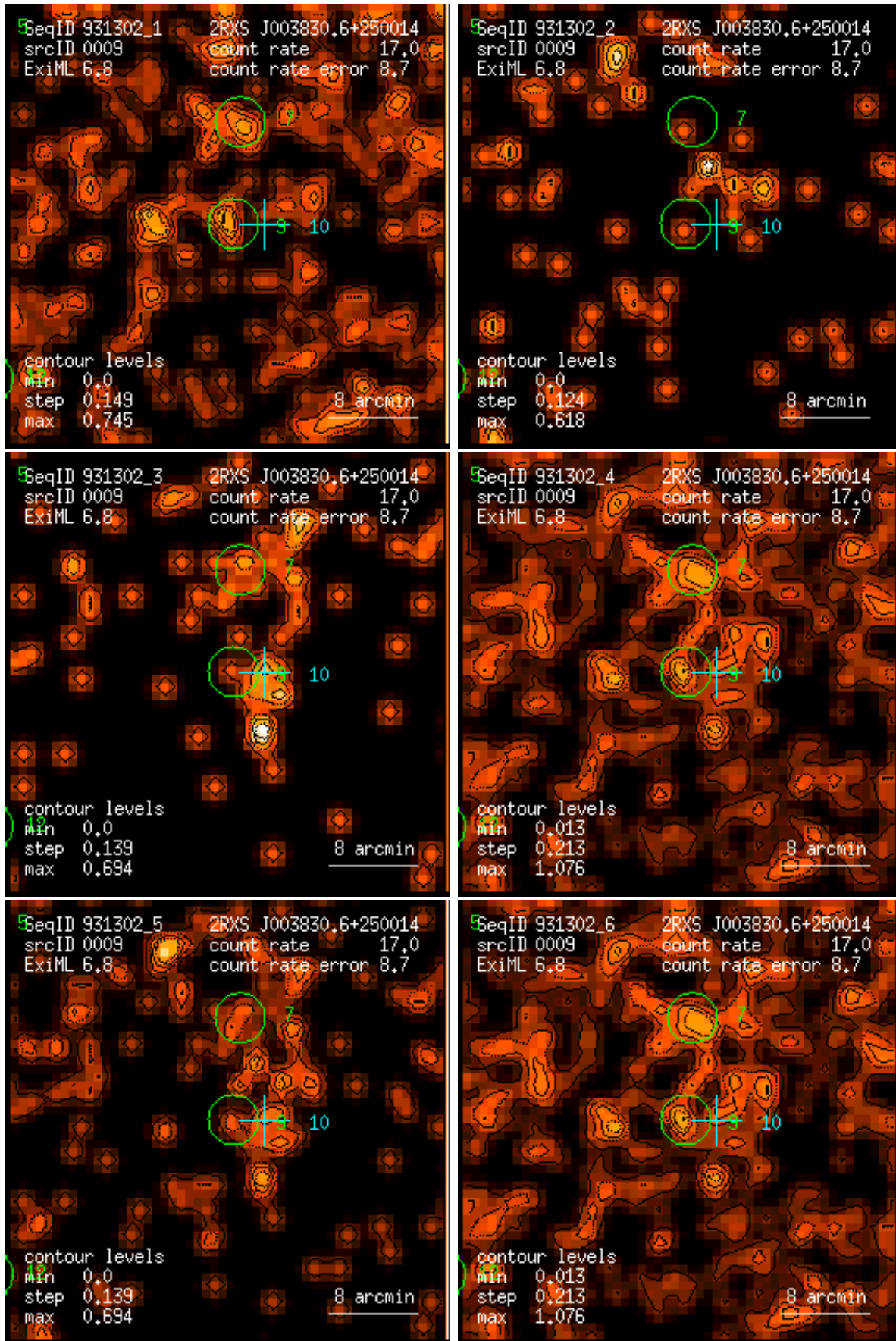
Figure 9: RASS 931302: detection 0009: band rate images, Gaussian filter: (1) PSPC channels 11 – 41, (2) 52 – 90, (3) 91 – 201, (4) 11 – 235, (5) 52 – 201, (6) 11 – 201. Broad band rates in counts/ks. Band rate contour levels in counts/ks/arcmin 2 .
