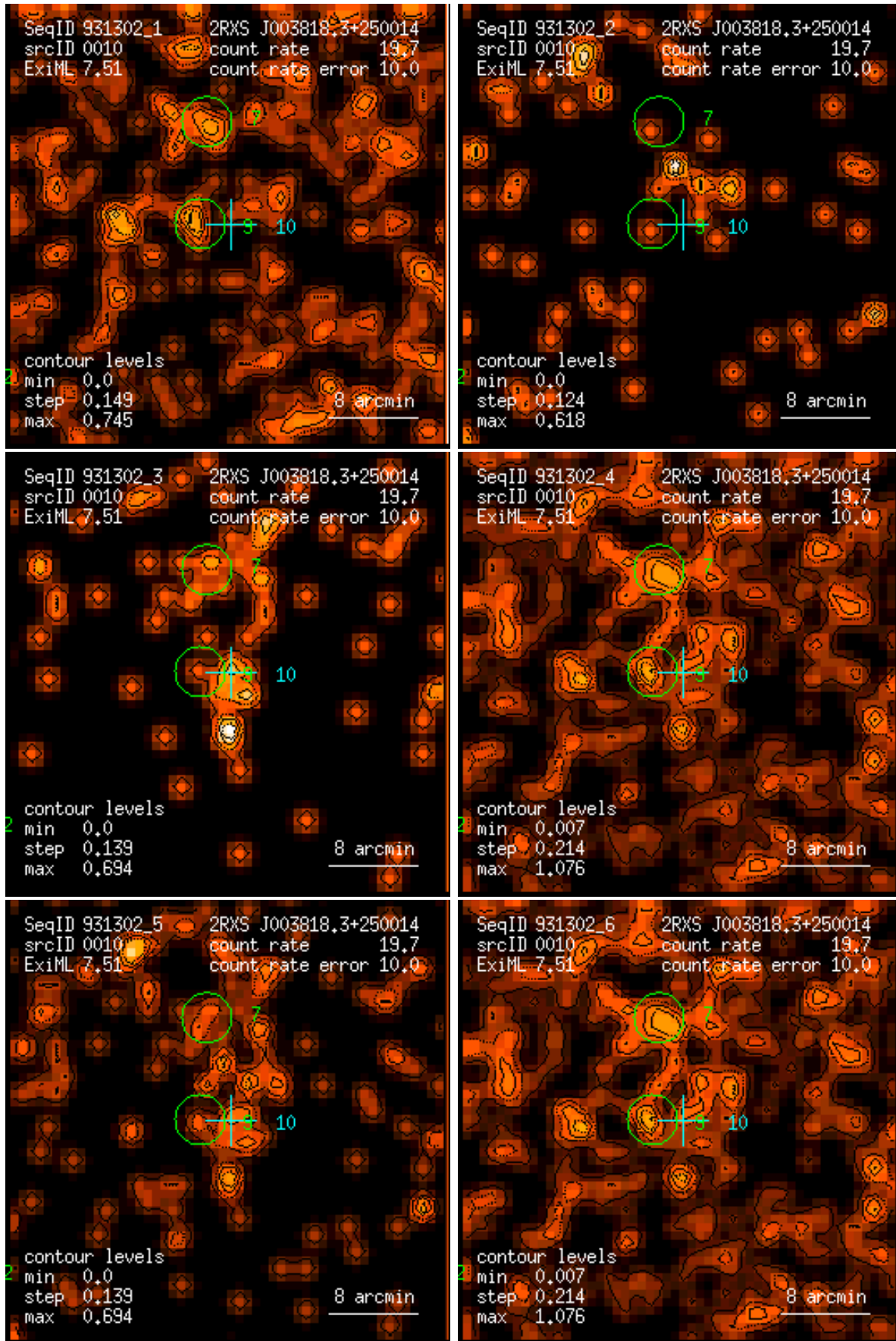
Figure 10: RASS 931302: detection 0010: band rate images, Gaussian filter: (1) PSPC channels 11 – 41, (2) 52 – 90, (3) 91 – 201, (4) 11 – 235, (5) 52 – 201, (6) 11 – 201. Broad band rates in counts/ks. Band rate contour levels in counts/ks/arcmin 2 .
