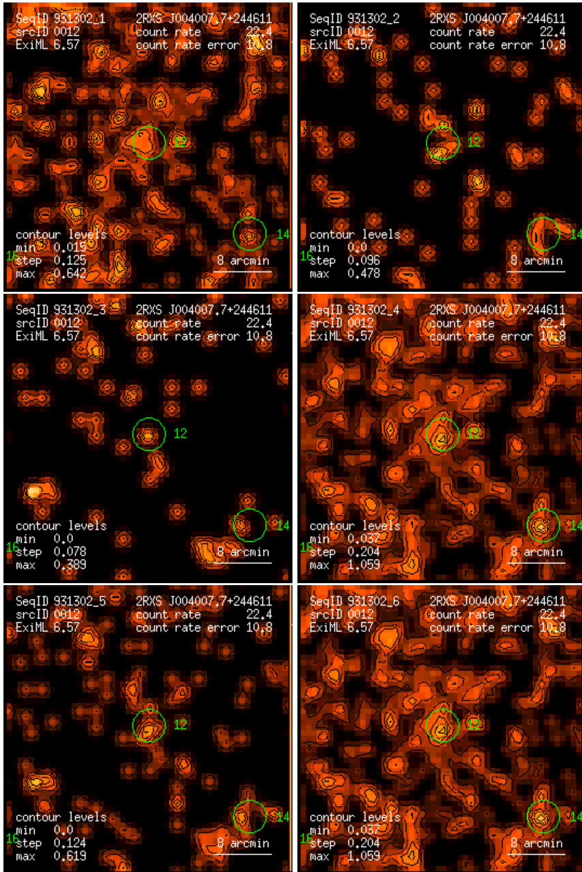
Figure 12: RASS 931302: detection 0012: band rate images, Gaussian filter: (1) PSPC channels 11 – 41, (2) 52 – 90, (3) 91 – 201, (4) 11 – 235, (5) 52 – 201, (6) 11 – 201. Broad band rates in counts/ks. Band rate contour levels in counts/ks/arcmin 2 .
