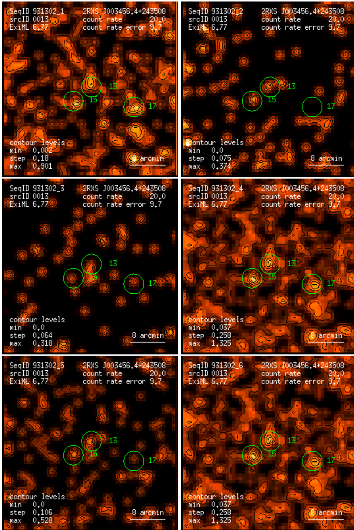
Figure 13: RASS 931302: detection 0013: band rate images, Gaussian filter: (1) PSPC channels 11 – 41, (2) 52 – 90, (3) 91 – 201, (4) 11 – 235, (5) 52 – 201, (6) 11 – 201. Broad band rates in counts/ks. Band rate contour levels in counts/ks/arcmin 2 .
