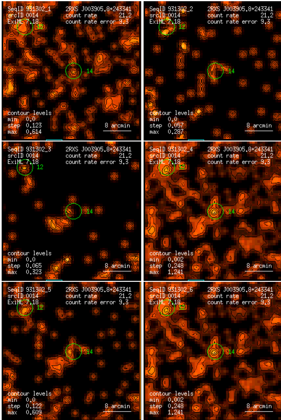
Figure 14: RASS 931302: detection 0014: band rate images, Gaussian filter: (1) PSPC channels 11 – 41, (2) 52 – 90, (3) 91 – 201, (4) 11 – 235, (5) 52 – 201, (6) 11 – 201. Broad band rates in counts/ks. Band rate contour levels in counts/ks/arcmin 2 .
