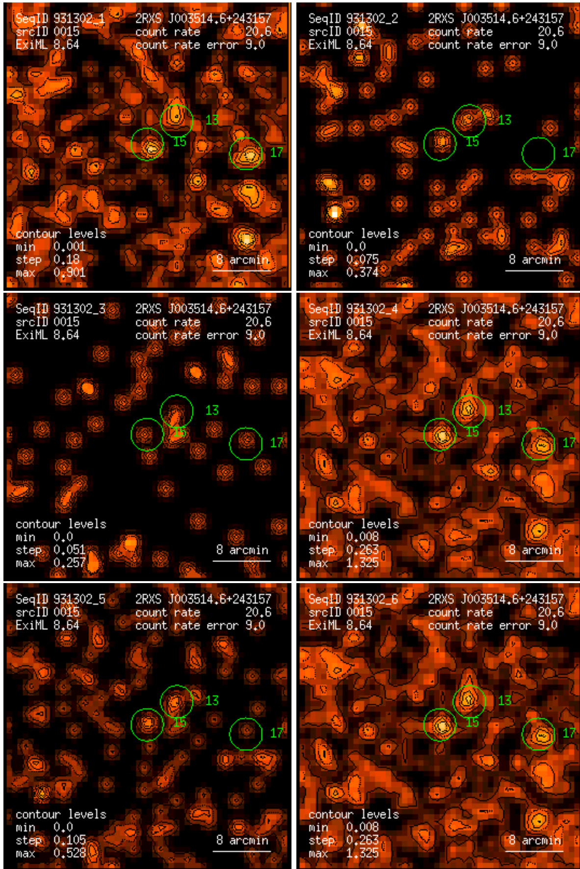
Figure 15: RASS 931302: detection 0015: band rate images, Gaussian filter: (1) PSPC channels 11 – 41, (2) 52 – 90, (3) 91 – 201, (4) 11 – 235, (5) 52 – 201, (6) 11 – 201. Broad band rates in counts/ks. Band rate contour levels in counts/ks/arcmin 2 .
