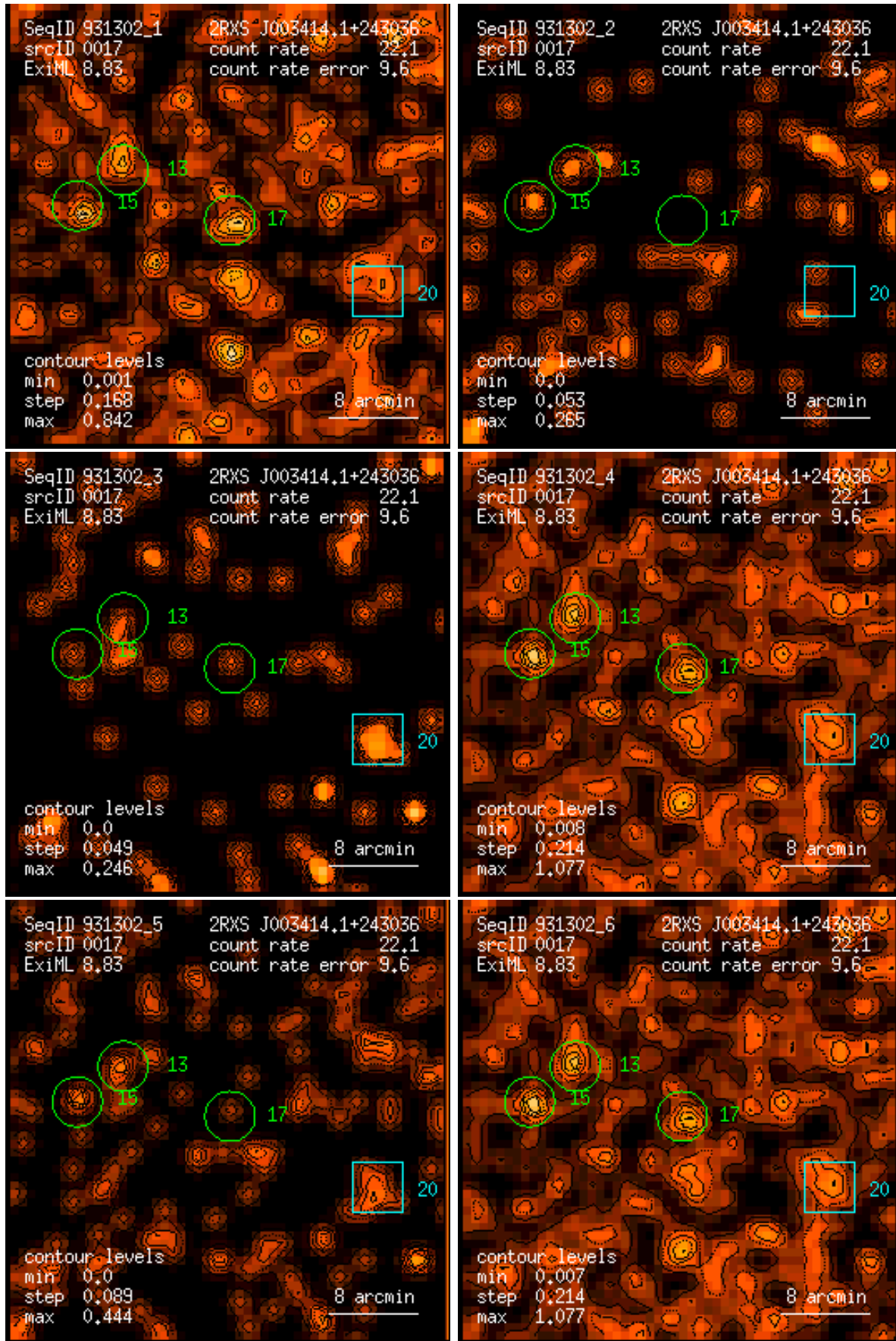
Figure 17: RASS 931302: detection 0017: band rate images, Gaussian filter: (1) PSPC channels 11 – 41, (2) 52 – 90, (3) 91 – 201, (4) 11 – 235, (5) 52 – 201, (6) 11 – 201. Broad band rates in counts/ks. Band rate contour levels in counts/ks/arcmin 2 .
