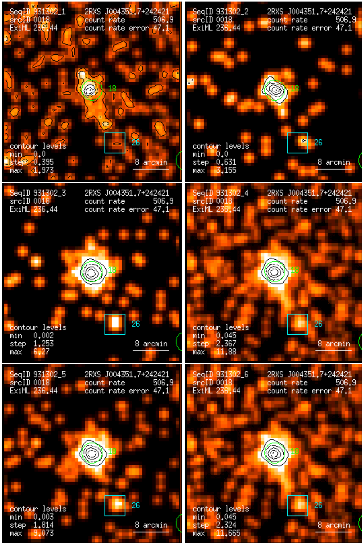
Figure 18: RASS 931302: detection 0018: band rate images, Gaussian filter: (1) PSPC channels 11 – 41, (2) 52 – 90, (3) 91 – 201, (4) 11 – 235, (5) 52 – 201, (6) 11 – 201. Broad band rates in counts/ks. Band rate contour levels in counts/ks/arcmin 2 .
