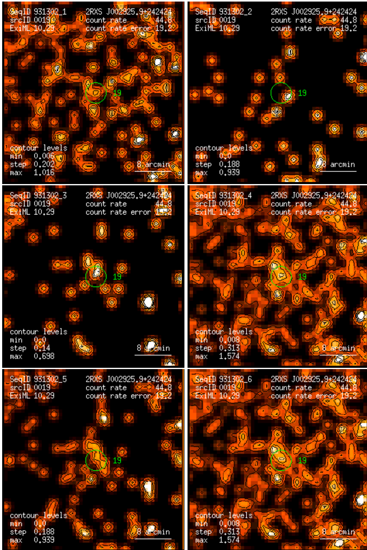
Figure 19: RASS 931302: detection 0019: band rate images, Gaussian filter: (1) PSPC channels 11 – 41, (2) 52 – 90, (3) 91 – 201, (4) 11 – 235, (5) 52 – 201, (6) 11 – 201. Broad band rates in counts/ks. Band rate contour levels in counts/ks/arcmin 2 .
