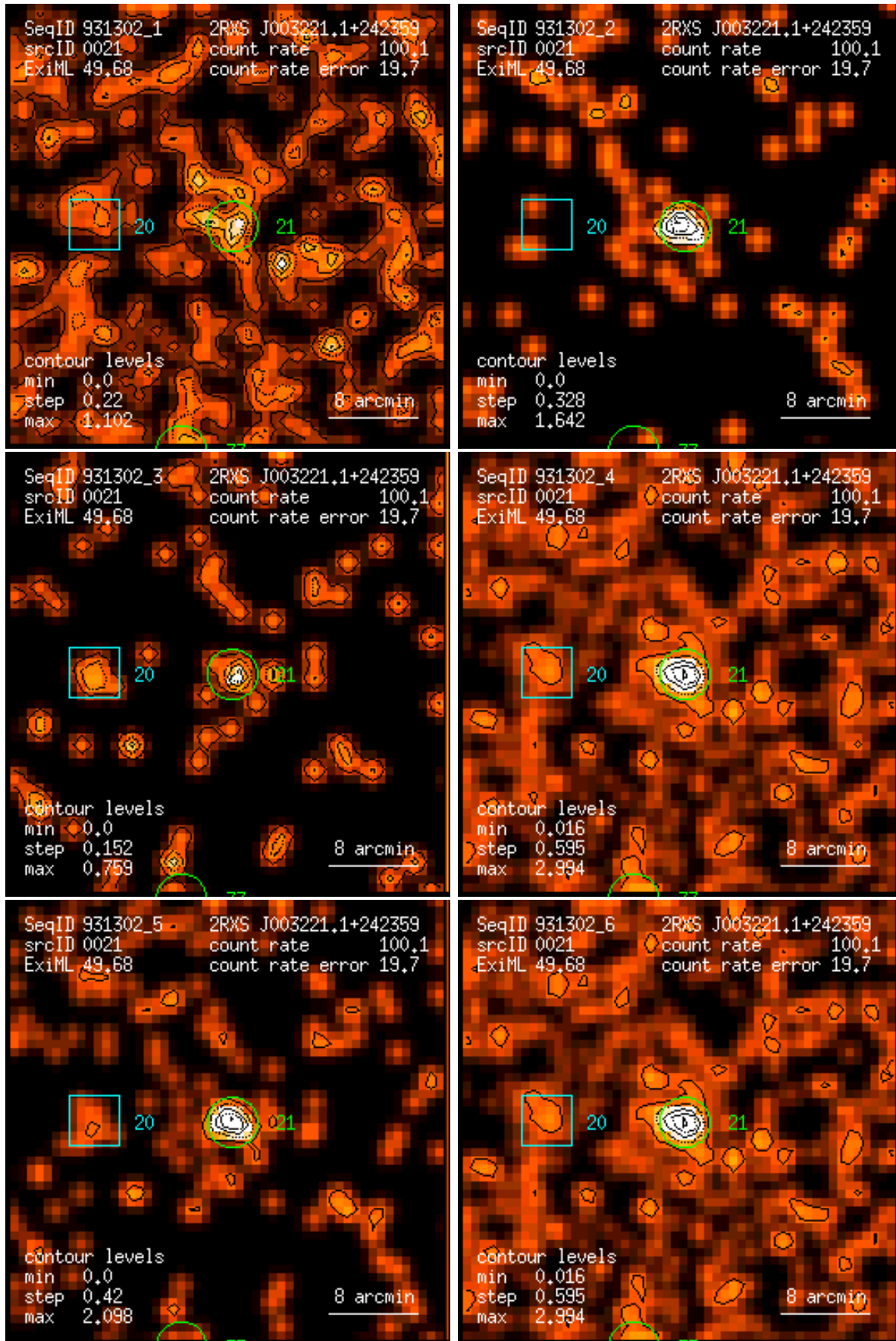
Figure 21: RASS 931302: detection 0021: band rate images, Gaussian filter: (1) PSPC channels 11 – 41, (2) 52 – 90, (3) 91 – 201, (4) 11 – 235, (5) 52 – 201, (6) 11 – 201. Broad band rates in counts/ks. Band rate contour levels in counts/ks/arcmin 2 .
