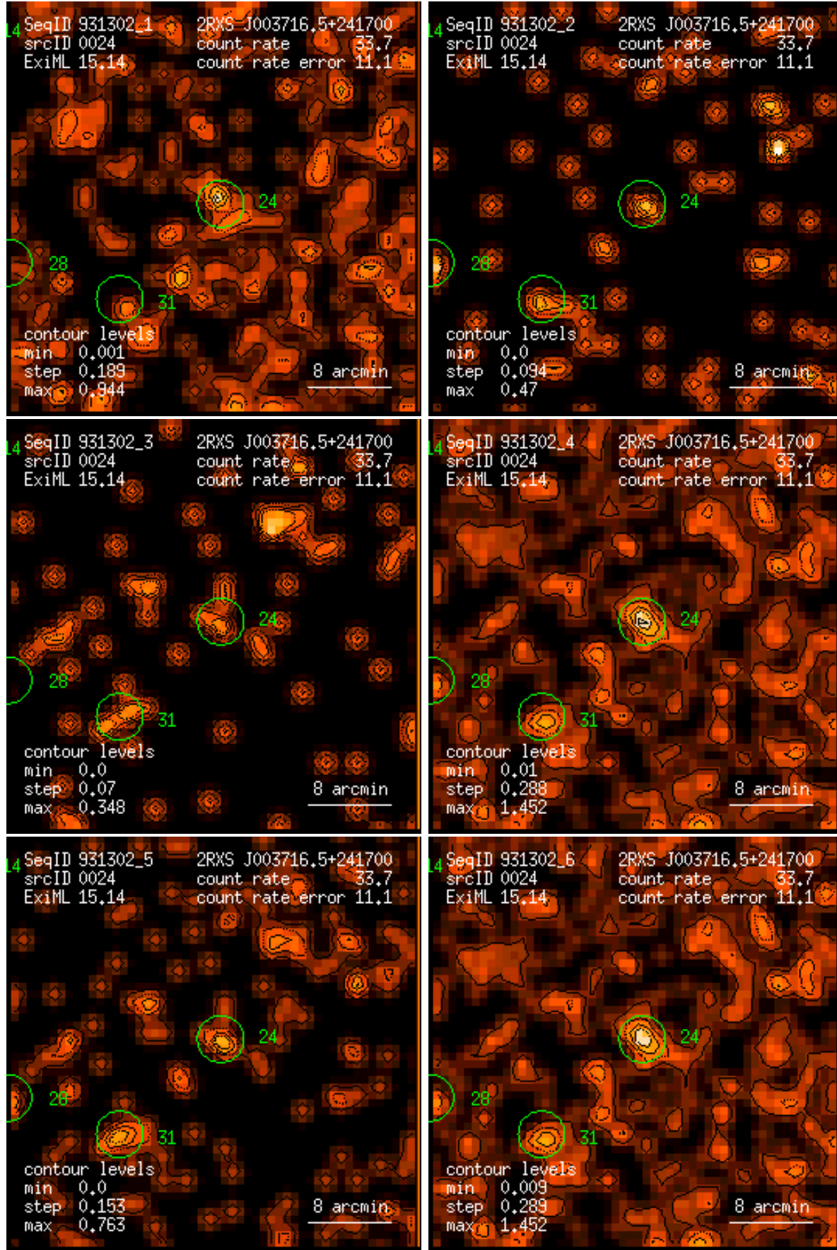
Figure 24: RASS 931302: detection 0024: band rate images, Gaussian filter: (1) PSPC channels 11 – 41, (2) 52 – 90, (3) 91 – 201, (4) 11 – 235, (5) 52 – 201, (6) 11 – 201. Broad band rates in counts/ks. Band rate contour levels in counts/ks/arcmin 2 .
