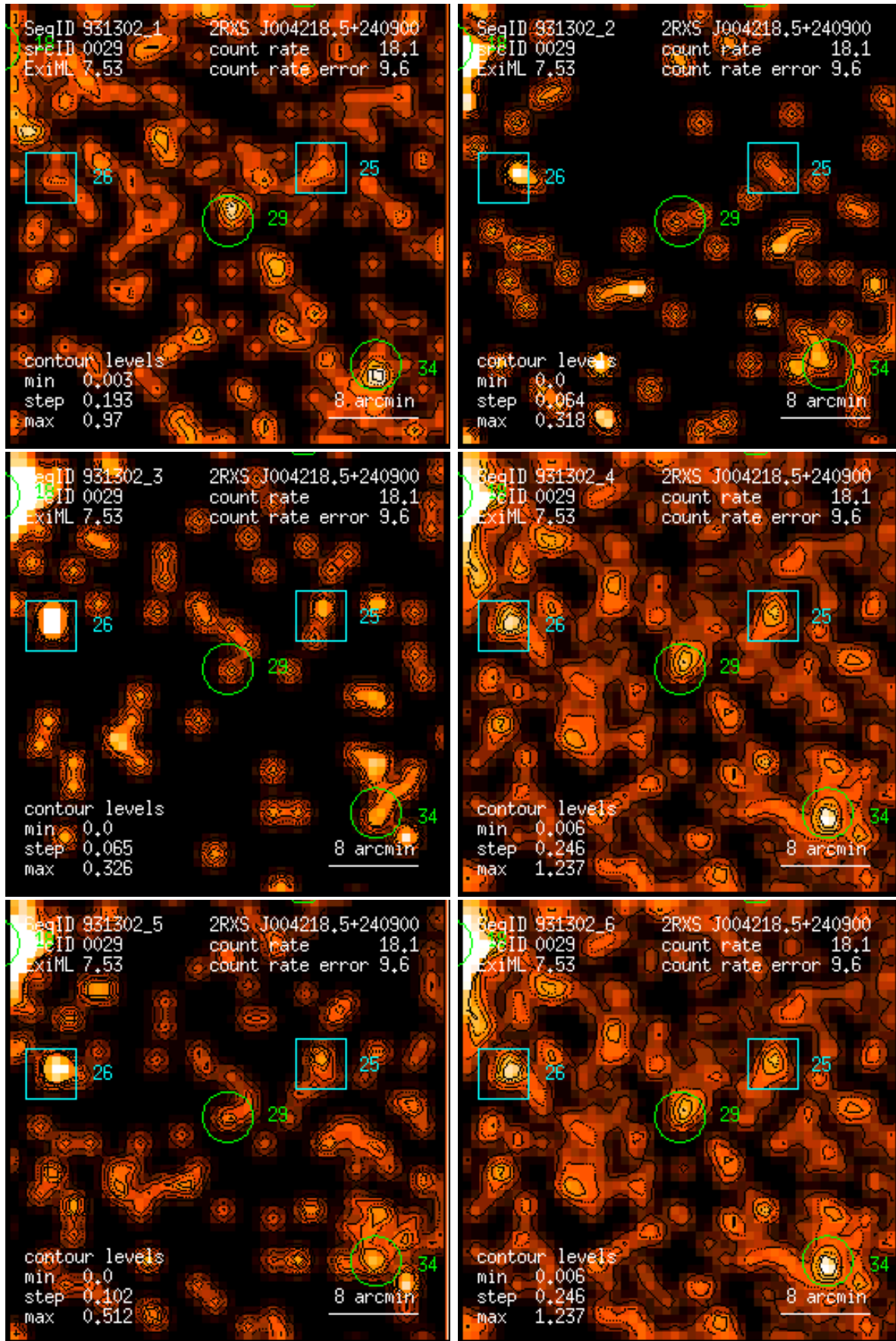
Figure 29: RASS 931302: detection 0029: band rate images, Gaussian filter: (1) PSPC channels 11 – 41, (2) 52 – 90, (3) 91 – 201, (4) 11 – 235, (5) 52 – 201, (6) 11 – 201. Broad band rates in counts/ks. Band rate contour levels in counts/ks/arcmin 2 .
