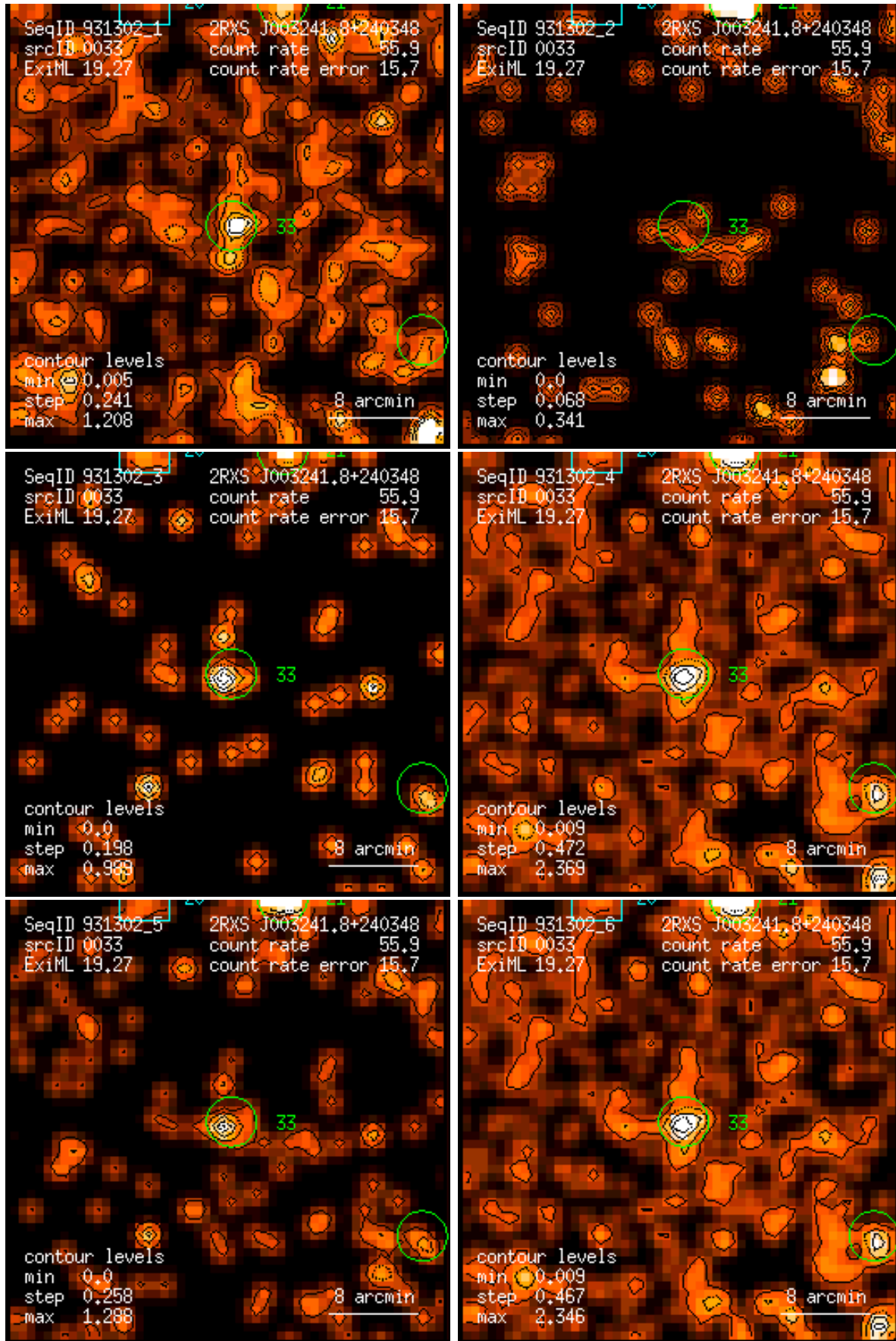
Figure 33: RASS 931302: detection 0033: band rate images, Gaussian filter: (1) PSPC channels 11 – 41, (2) 52 – 90, (3) 91 – 201, (4) 11 – 235, (5) 52 – 201, (6) 11 – 201. Broad band rates in counts/ks. Band rate contour levels in counts/ks/arcmin 2 .
