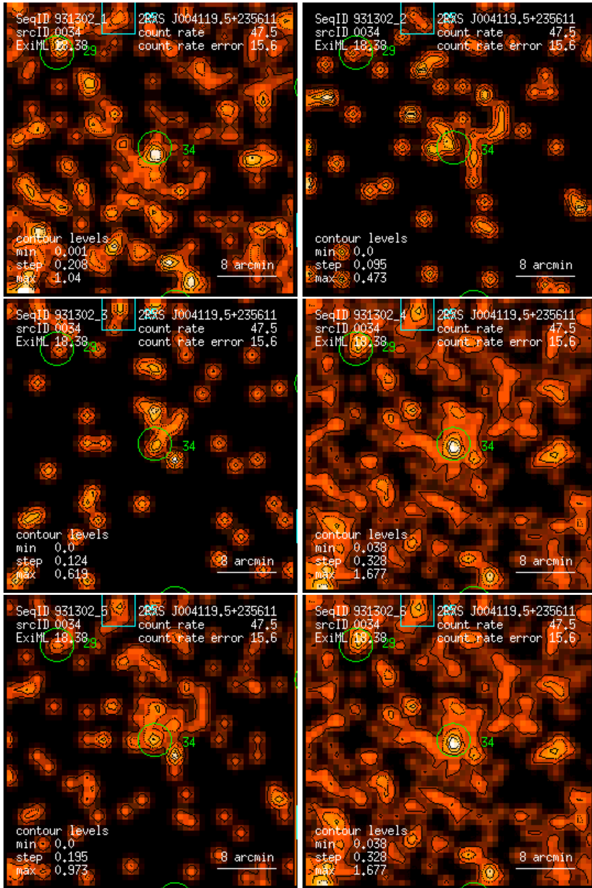
Figure 34: RASS 931302: detection 0034: band rate images, Gaussian filter: (1) PSPC channels 11 – 41, (2) 52 – 90, (3) 91 – 201, (4) 11 – 235, (5) 52 – 201, (6) 11 – 201. Broad band rates in counts/ks. Band rate contour levels in counts/ks/arcmin 2 .
