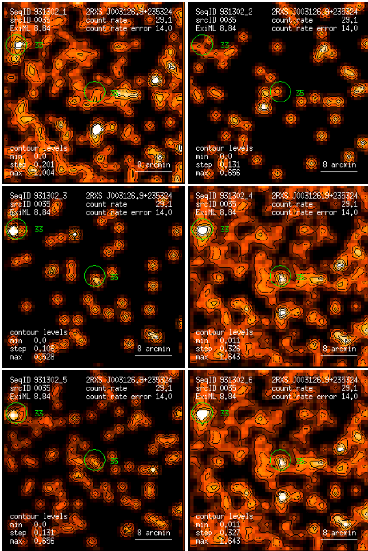
Figure 35: RASS 931302: detection 0035: band rate images, Gaussian filter: (1) PSPC channels 11 – 41, (2) 52 – 90, (3) 91 – 201, (4) 11 – 235, (5) 52 – 201, (6) 11 – 201. Broad band rates in counts/ks. Band rate contour levels in counts/ks/arcmin 2 .
