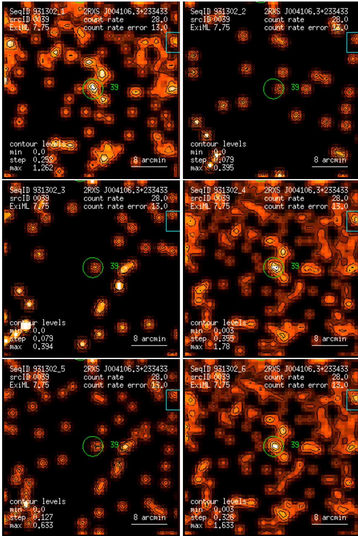
Figure 39: RASS 931302: detection 0039: band rate images, Gaussian filter: (1) PSPC channels 11 – 41, (2) 52 – 90, (3) 91 – 201, (4) 11 – 235, (5) 52 – 201, (6) 11 – 201. Broad band rates in counts/ks. Band rate contour levels in counts/ks/arcmin 2 .
