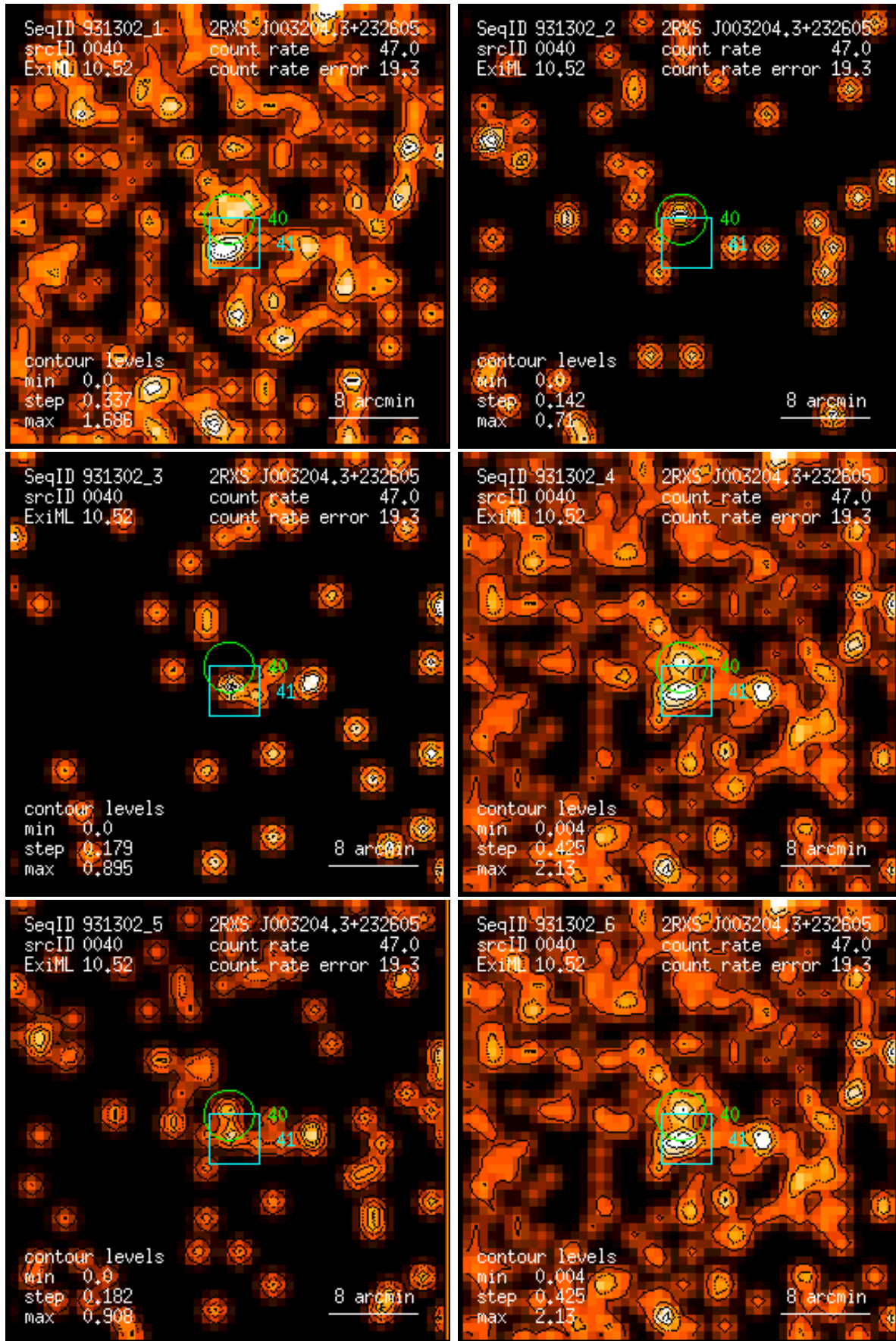
Figure 40: RASS 931302: detection 0040: band rate images, Gaussian filter: (1) PSPC channels 11 – 41, (2) 52 – 90, (3) 91 – 201, (4) 11 – 235, (5) 52 – 201, (6) 11 – 201. Broad band rates in counts/ks. Band rate contour levels in counts/ks/arcmin 2 .
