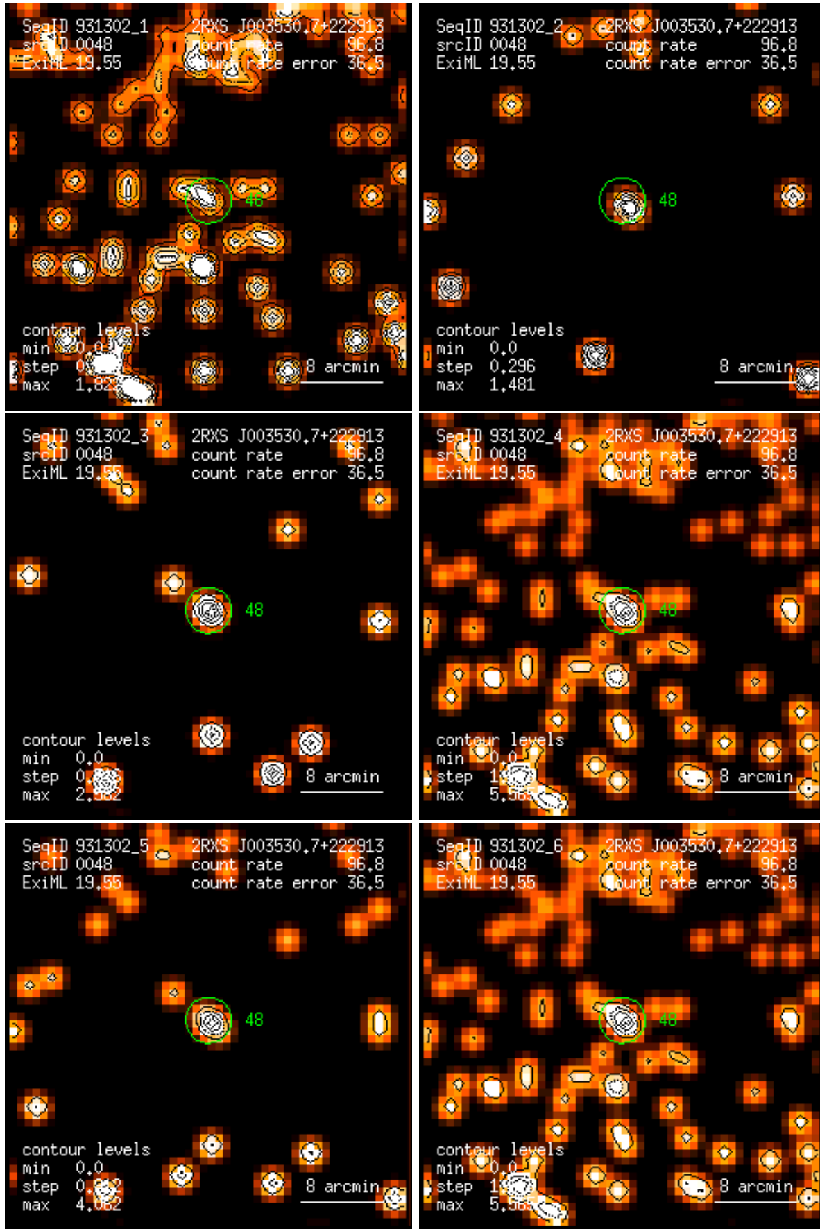
Figure 48: RASS 931302: detection 0048: band rate images, Gaussian filter: (1) PSPC channels 11 – 41, (2) 52 – 90, (3) 91 – 201, (4) 11 – 235, (5) 52 – 201, (6) 11 – 201. Broad band rates in counts/ks. Band rate contour levels in counts/ks/arcmin 2 .
