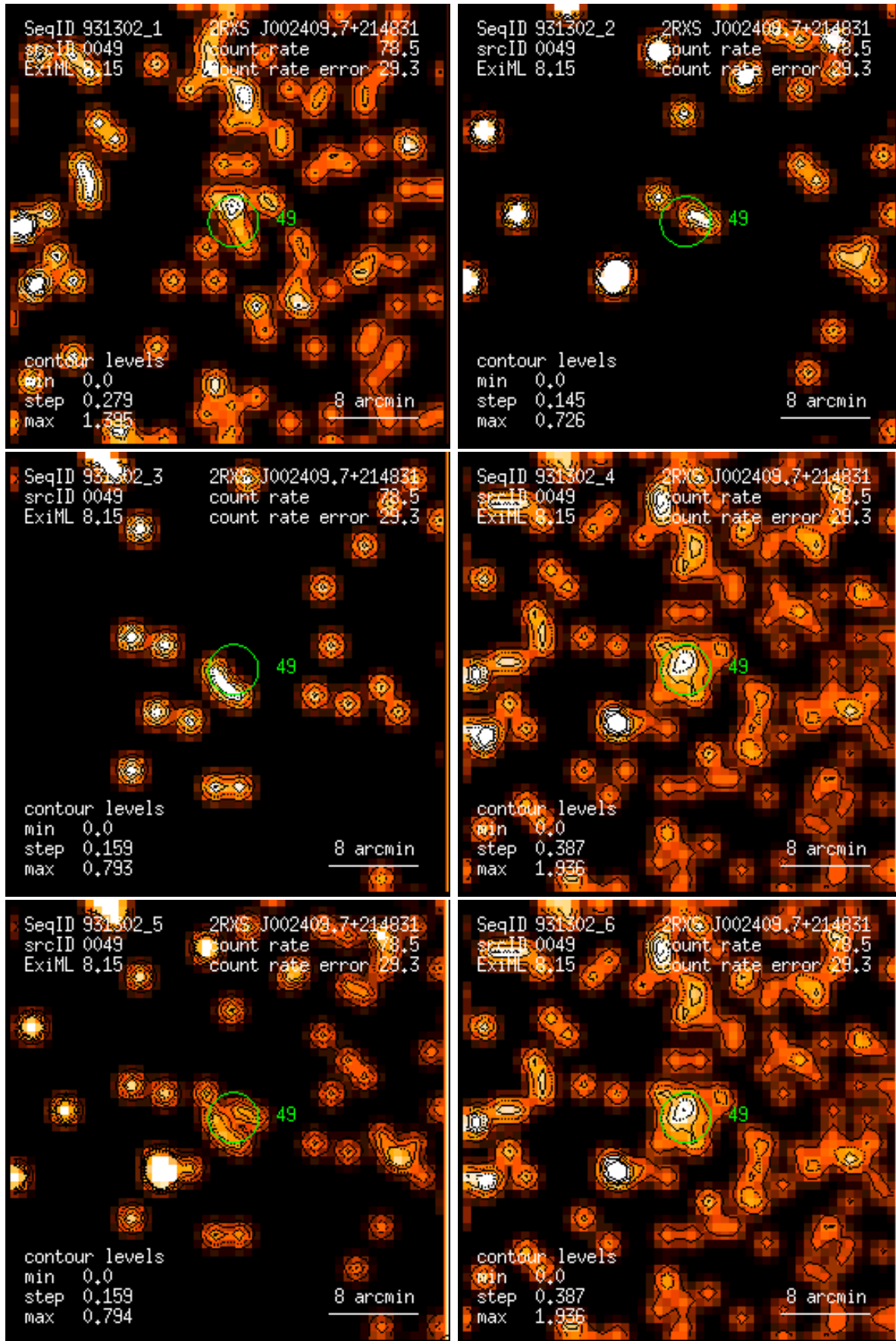
Figure 49: RASS 931302: detection 0049: band rate images, Gaussian filter: (1) PSPC channels 11 – 41, (2) 52 – 90, (3) 91 – 201, (4) 11 – 235, (5) 52 – 201, (6) 11 – 201. Broad band rates in counts/ks. Band rate contour levels in counts/ks/arcmin 2 .
