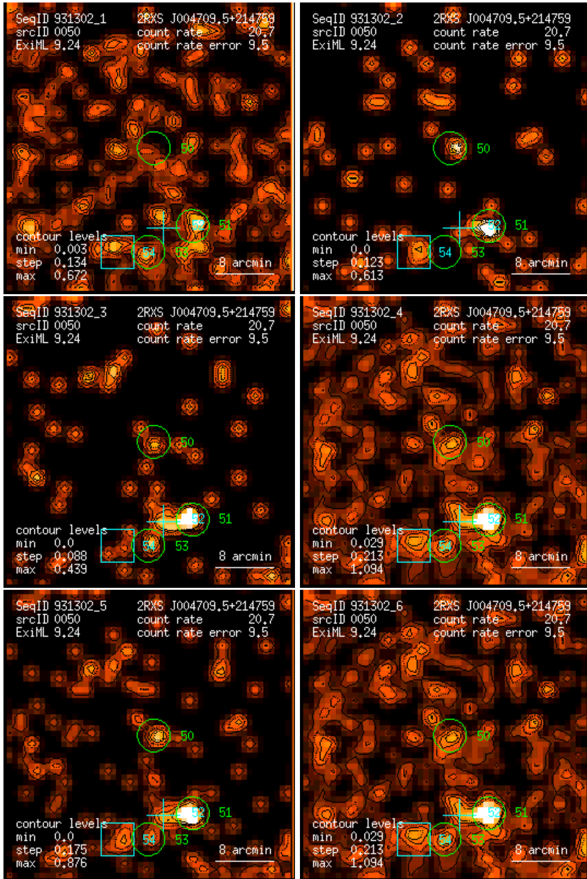
Figure 50: RASS 931302: detection 0050: band rate images, Gaussian filter: (1) PSPC channels 11 – 41, (2) 52 – 90, (3) 91 – 201, (4) 11 – 235, (5) 52 – 201, (6) 11 – 201. Broad band rates in counts/ks. Band rate contour levels in counts/ks/arcmin 2 .
