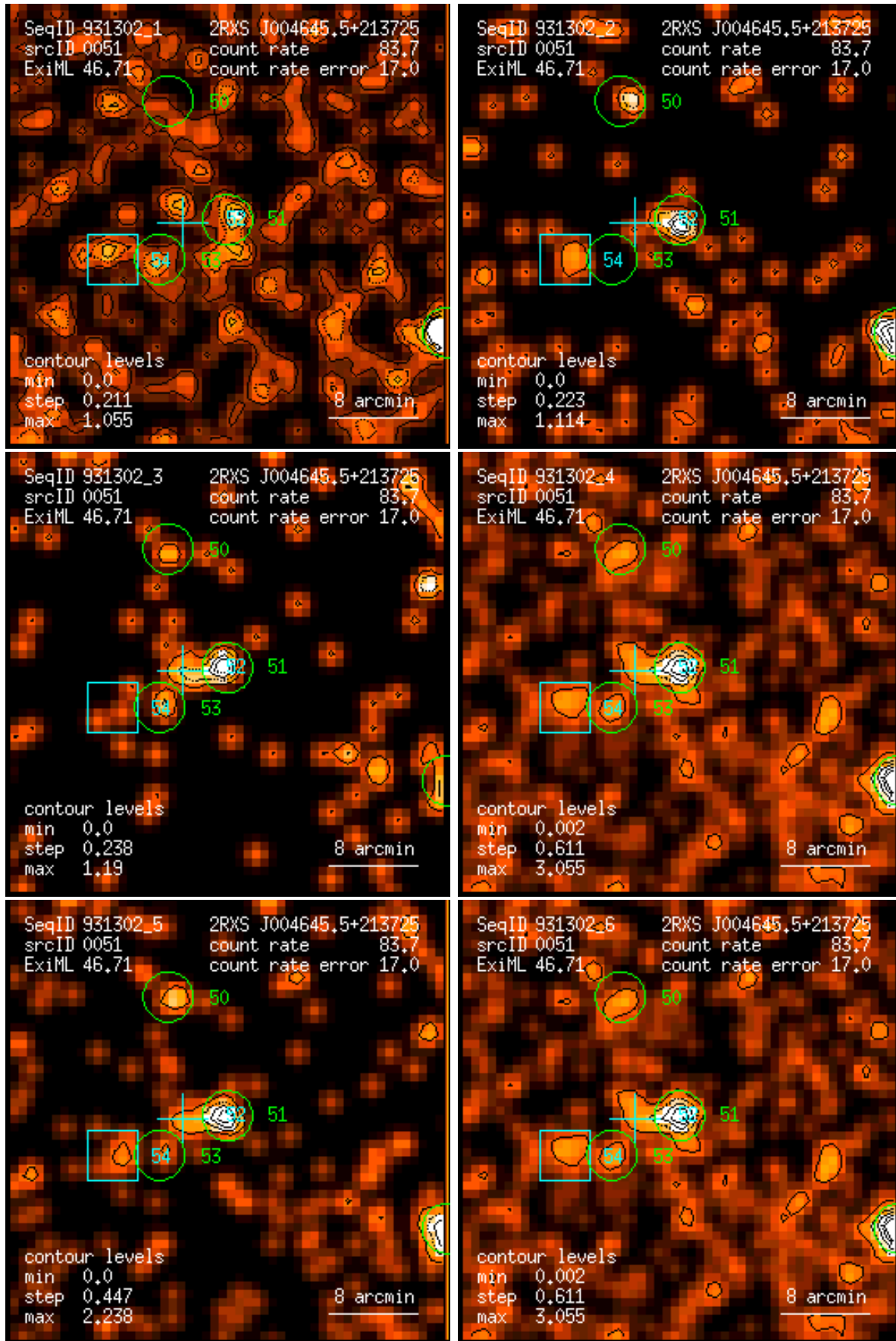
Figure 51: RASS 931302: detection 0051: band rate images, Gaussian filter: (1) PSPC channels 11 – 41, (2) 52 – 90, (3) 91 – 201, (4) 11 – 235, (5) 52 – 201, (6) 11 – 201. Broad band rates in counts/ks. Band rate contour levels in counts/ks/arcmin 2 .
