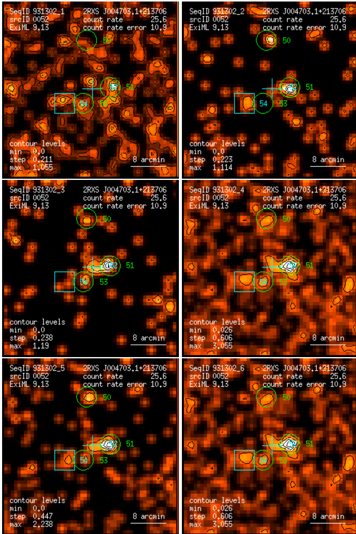
Figure 52: RASS 931302: detection 0052: band rate images, Gaussian filter: (1) PSPC channels 11 – 41, (2) 52 – 90, (3) 91 – 201, (4) 11 – 235, (5) 52 – 201, (6) 11 – 201. Broad band rates in counts/ks. Band rate contour levels in counts/ks/arcmin 2 .
