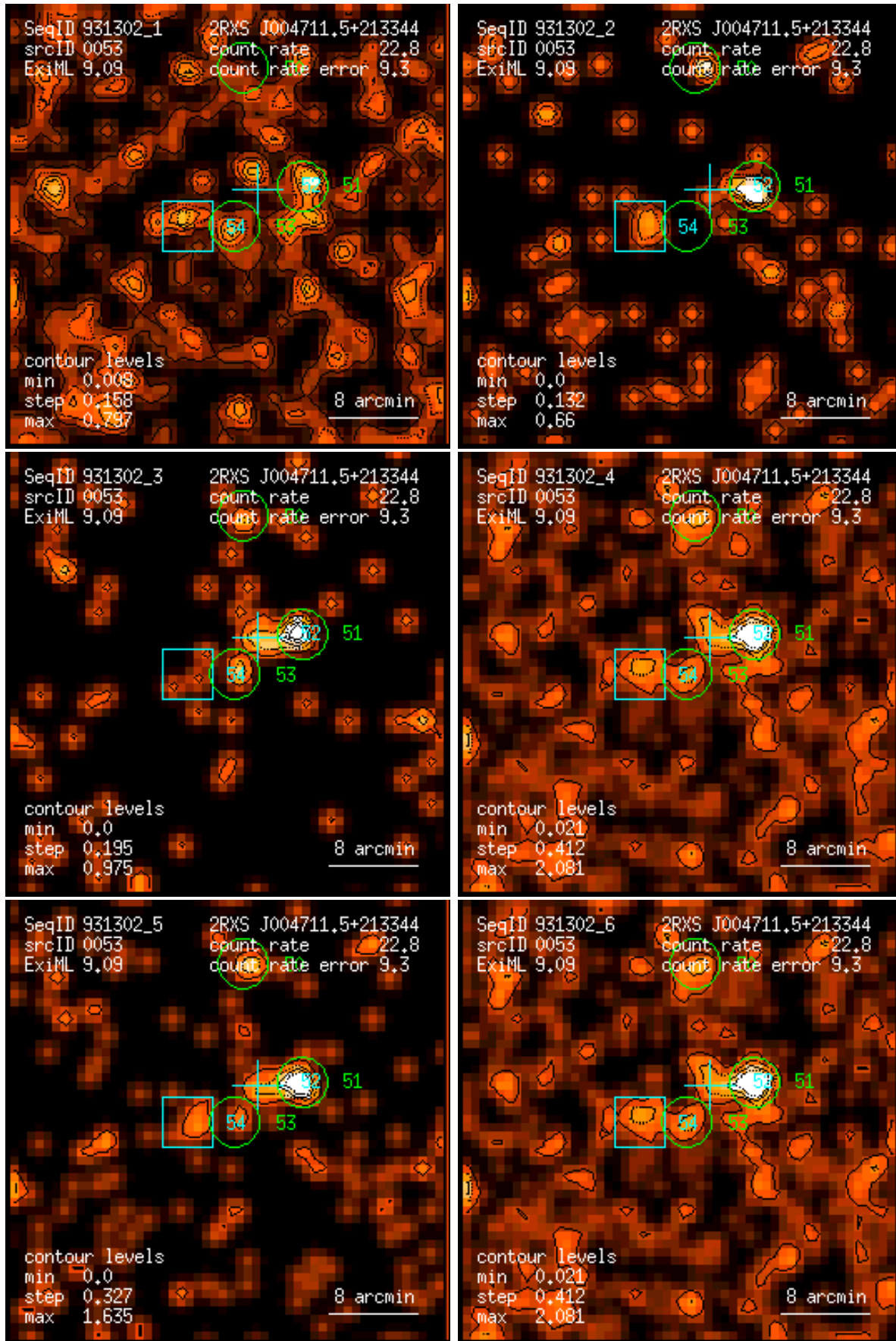
Figure 53: RASS 931302: detection 0053: band rate images, Gaussian filter: (1) PSPC channels 11 – 41, (2) 52 – 90, (3) 91 – 201, (4) 11 – 235, (5) 52 – 201, (6) 11 – 201. Broad band rates in counts/ks. Band rate contour levels in counts/ks/arcmin 2 .
