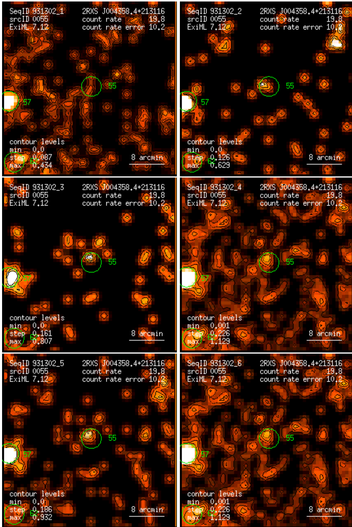
Figure 55: RASS 931302: detection 0055: band rate images, Gaussian filter: (1) PSPC channels 11 – 41, (2) 52 – 90, (3) 91 – 201, (4) 11 – 235, (5) 52 – 201, (6) 11 – 201. Broad band rates in counts/ks. Band rate contour levels in counts/ks/arcmin 2 .
