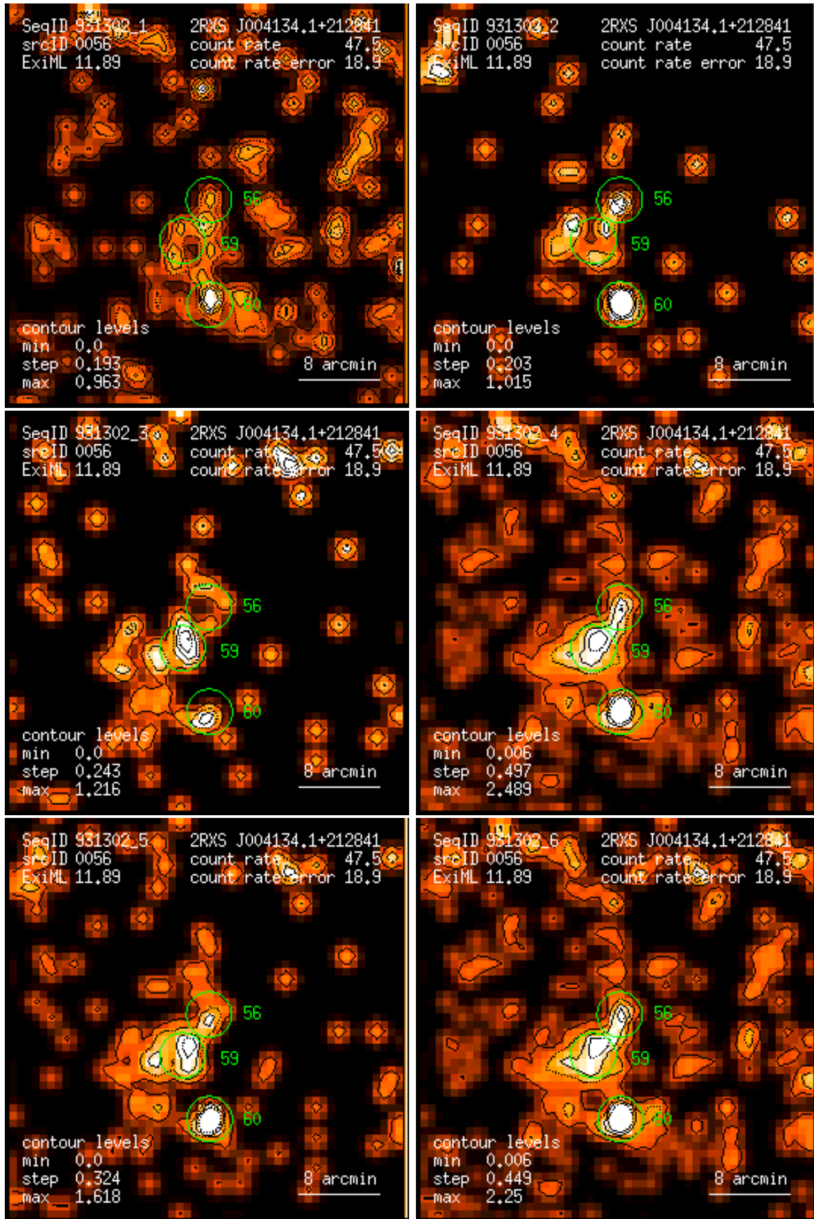
Figure 56: RASS 931302: detection 0056: band rate images, Gaussian filter: (1) PSPC channels 11 – 41, (2) 52 – 90, (3) 91 – 201, (4) 11 – 235, (5) 52 – 201, (6) 11 – 201. Broad band rates in counts/ks. Band rate contour levels in counts/ks/arcmin 2 .
