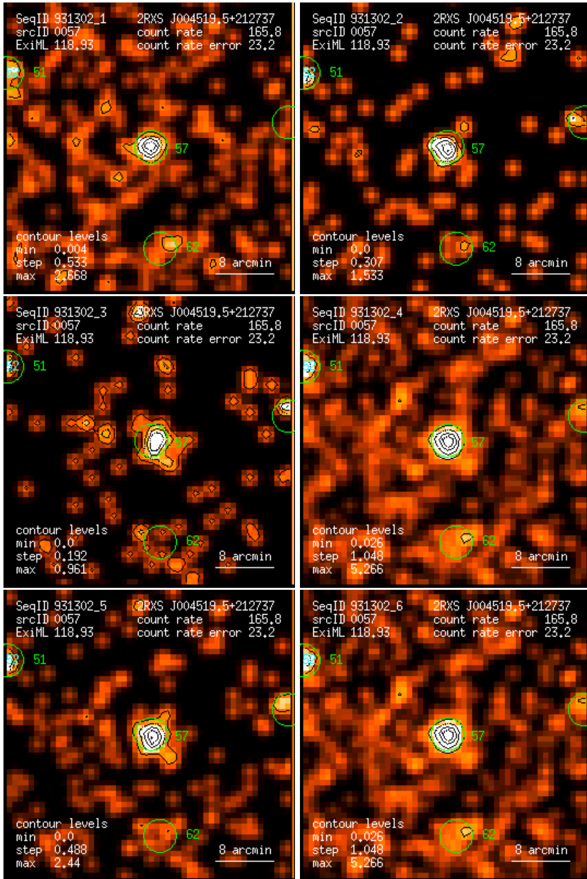
Figure 57: RASS 931302: detection 0057: band rate images, Gaussian filter: (1) PSPC channels 11 – 41, (2) 52 – 90, (3) 91 – 201, (4) 11 – 235, (5) 52 – 201, (6) 11 – 201. Broad band rates in counts/ks. Band rate contour levels in counts/ks/arcmin 2 .
