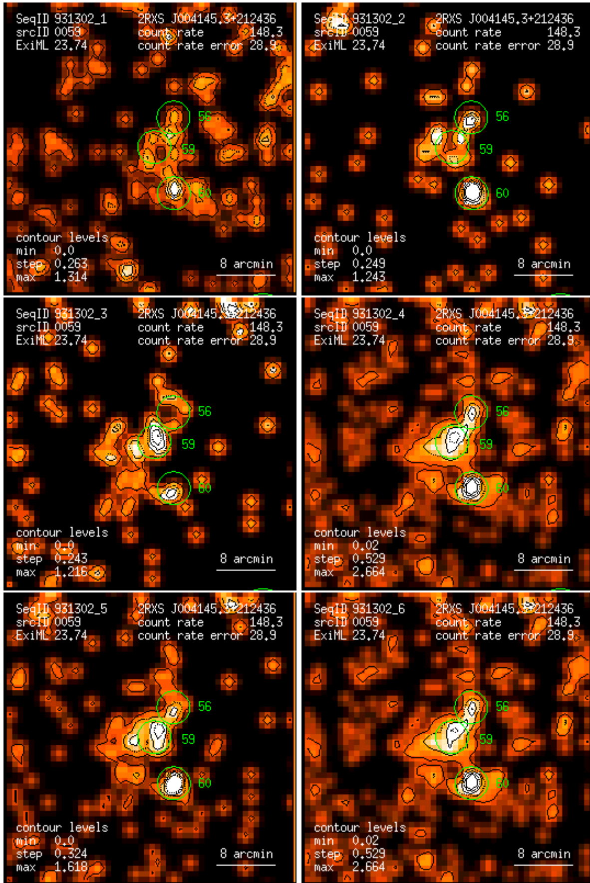
Figure 59: RASS 931302: detection 0059: band rate images, Gaussian filter: (1) PSPC channels 11 – 41, (2) 52 – 90, (3) 91 – 201, (4) 11 – 235, (5) 52 – 201, (6) 11 – 201. Broad band rates in counts/ks. Band rate contour levels in counts/ks/arcmin 2 .
