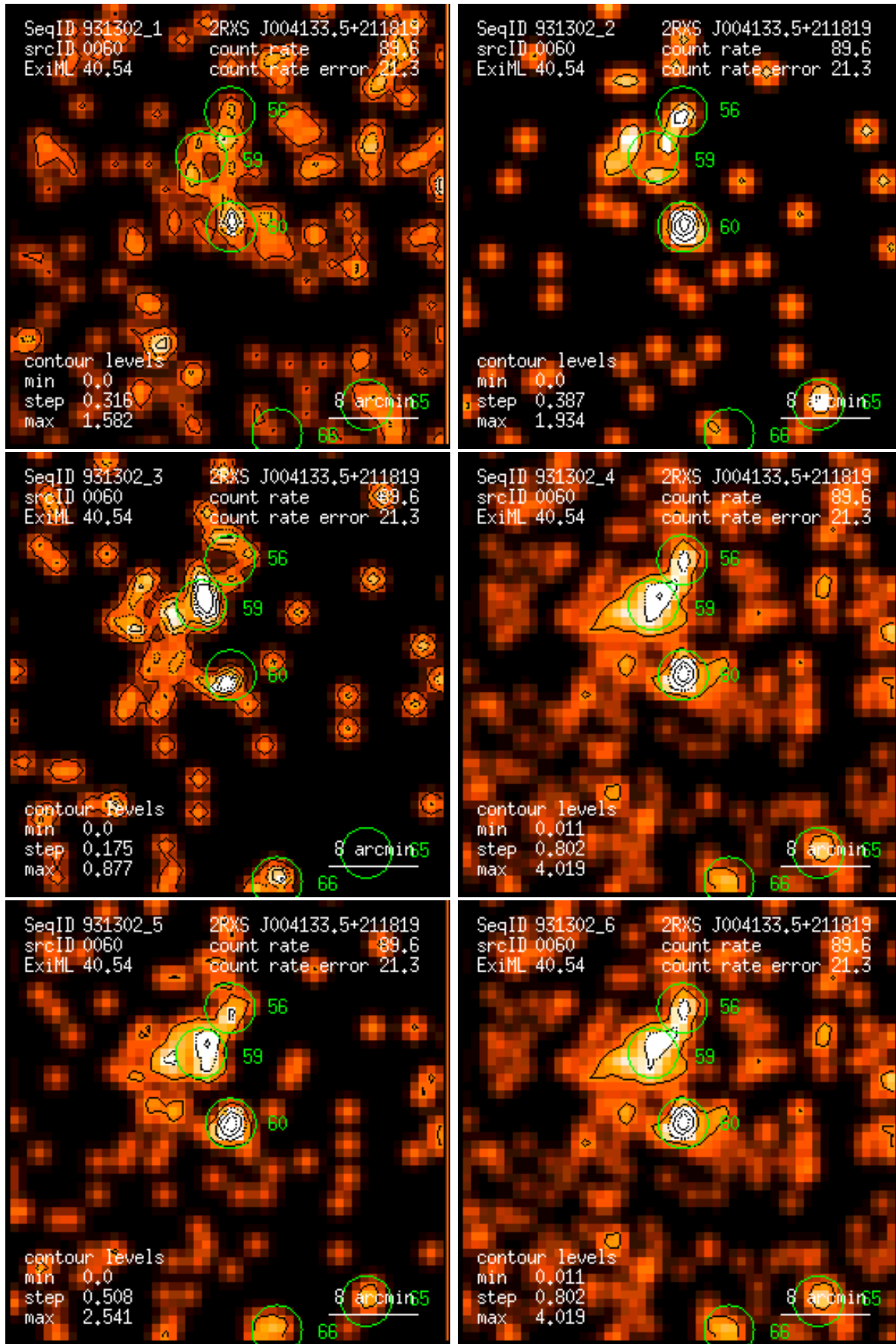
Figure 60: RASS 931302: detection 0060: band rate images, Gaussian filter: (1) PSPC channels 11 – 41, (2) 52 – 90, (3) 91 – 201, (4) 11 – 235, (5) 52 – 201, (6) 11 – 201. Broad band rates in counts/ks. Band rate contour levels in counts/ks/arcmin 2 .
