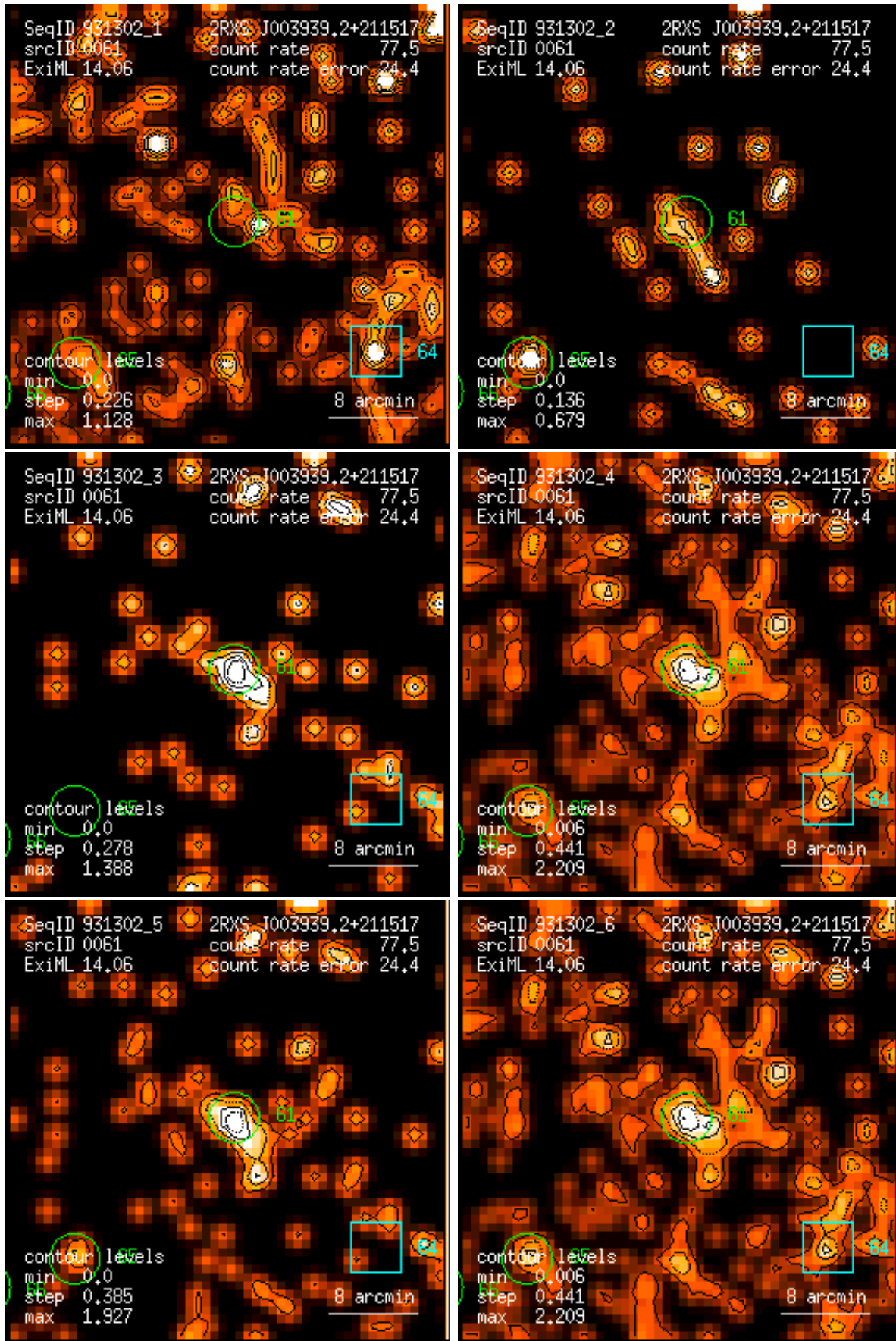
Figure 61: RASS 931302: detection 0061: band rate images, Gaussian filter: (1) PSPC channels 11 – 41, (2) 52 – 90, (3) 91 – 201, (4) 11 – 235, (5) 52 – 201, (6) 11 – 201. Broad band rates in counts/ks. Band rate contour levels in counts/ks/arcmin 2 .
