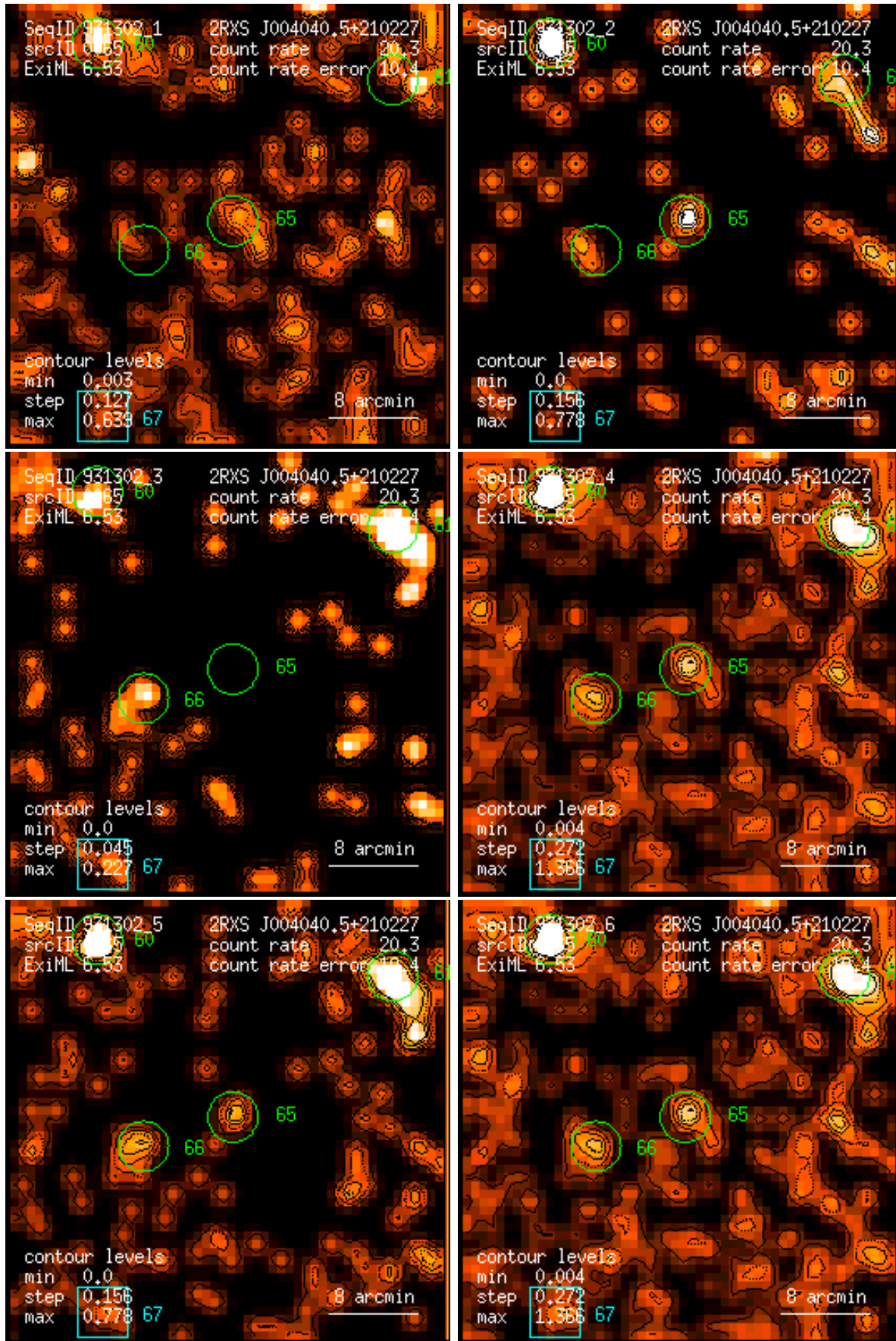
Figure 65: RASS 931302: detection 0065: band rate images, Gaussian filter: (1) PSPC channels 11 – 41, (2) 52 – 90, (3) 91 – 201, (4) 11 – 235, (5) 52 – 201, (6) 11 – 201. Broad band rates in counts/ks. Band rate contour levels in counts/ks/arcmin 2 .
