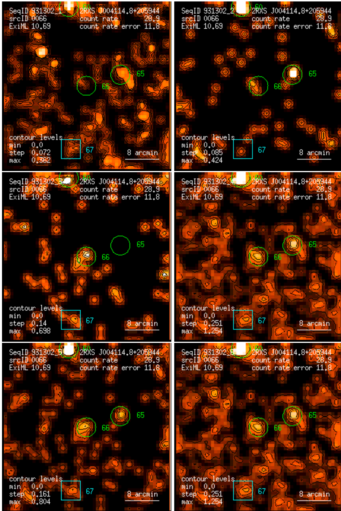
Figure 66: RASS 931302: detection 0066: band rate images, Gaussian filter: (1) PSPC channels 11 – 41, (2) 52 – 90, (3) 91 – 201, (4) 11 – 235, (5) 52 – 201, (6) 11 – 201. Broad band rates in counts/ks. Band rate contour levels in counts/ks/arcmin 2 .
