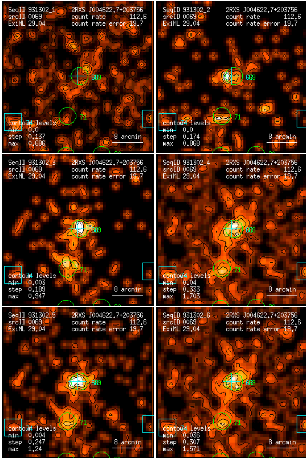
Figure 69: RASS 931302: detection 0069: band rate images, Gaussian filter: (1) PSPC channels 11 – 41, (2) 52 – 90, (3) 91 – 201, (4) 11 – 235, (5) 52 – 201, (6) 11 – 201. Broad band rates in counts/ks. Band rate contour levels in counts/ks/arcmin 2 .
